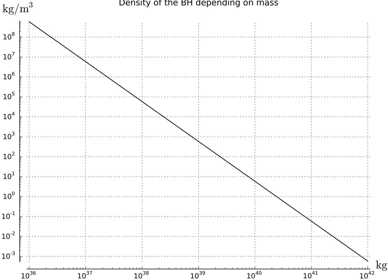
Density of the BH depending on mass
