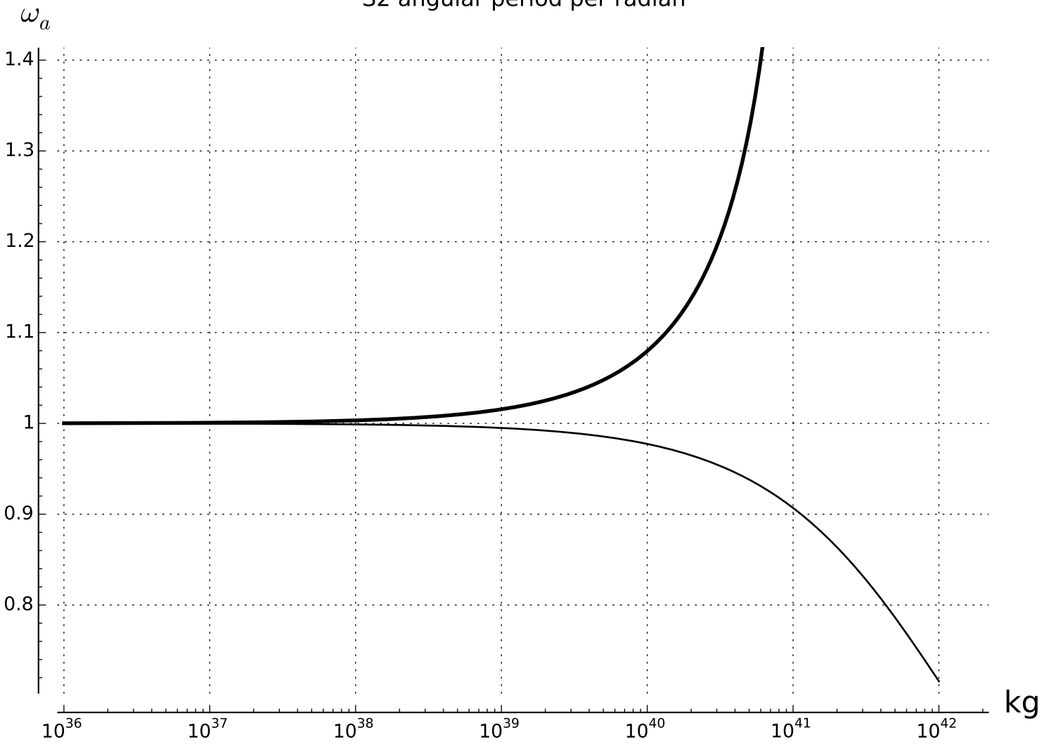
S2 angular period per radian
