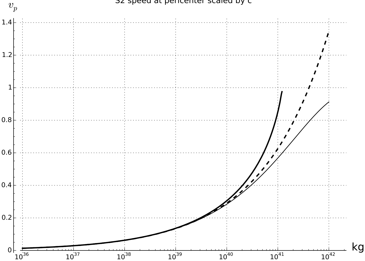
S2 speed at pericenter scaled by c
