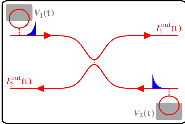
Figure 1 (Color online) HOM setup in the IQH regime. Two chiral edge channels meet at a QPC. Each one is coupled to a SES in the optimal regime of emission of electrons (holes). Current cross-correlations at the two outputs are measured at zero frequency as a function of the delay between the electron emissions. Picture taken from [13].
