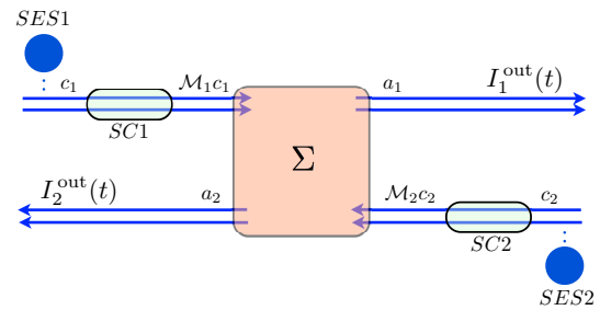
Figure 9 (Color online) QPC geometry for Bogoliubov quasiparticles. The individual electron sources SES1 and SES2 inject electrons (described by the operators c_j ( j = 1, 2 )), into the two SC contacts SC1 and SC2 . The outgoing excitation ( \mathcal{M}_j c_j ) reach the QPC and are partitioned according to the scattering matrix \Sigma . We consider the cross-correlated noise between the outgoing currents I_j^{out}(t) (written in terms of the operators a_j ). Picture taken from [19].
