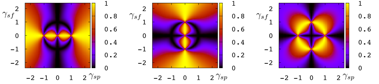
Figure 4 (Color on-line) Density plot of \mathcal{I} (left), \mathcal{J} (middle) and \mathcal{K} (right) as a function of \gamma_{sp} and \gamma_{sf} . Picture taken from [18].
