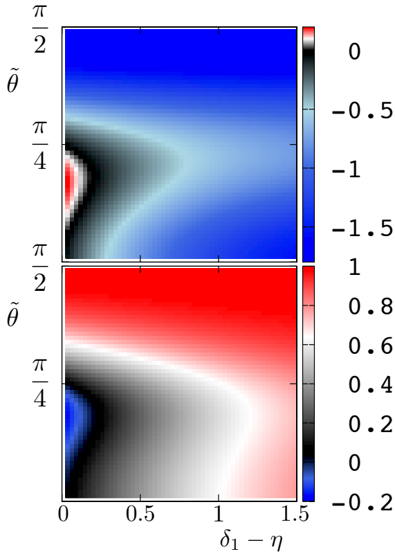
Figure 10 (Color online). Upper panel. Density plot of \mathcal{S}_{HOM}^{1SC} in units of \mathcal{S}_0 = e^2 \mathcal{R} T . “Blue” identifies negative regions where the hole contribution dominates over the electron one, while the little red area represents the positive noise. Lower panel. Density plot of R^{1SC} as a function of \delta_1 - \eta and \tilde{\theta} . The blue area corresponds to negative values of the ratio which cannot be reached in conventional electronic quantum optics experiments. Picture taken from [19].
