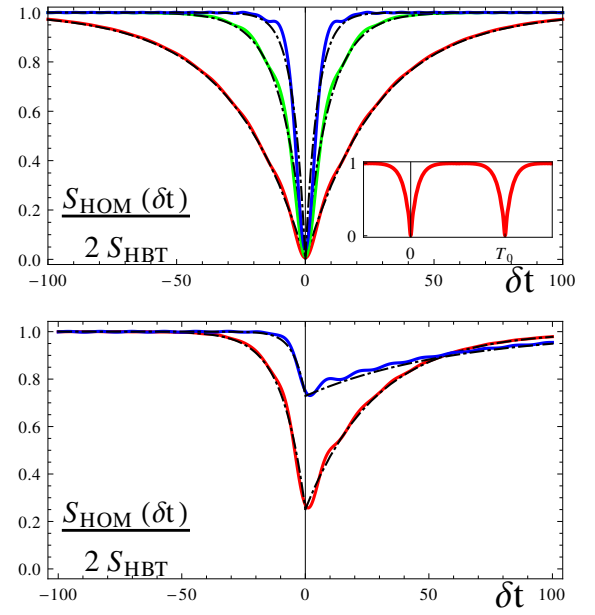
Figure 2 (Color online) Normalized HOM noise as a function of the delay in the electron (hole) emission \delta t . Full curves represent the result obtained within the Floquet scattering matrix formalism in the optimal emission regime of the SES. Dotted-dashed curves are the analytical predictions of Eq. (10) for exponential WPs. Upper panel: symmetric profile, with emitter transparencies D = 0.2 (red curve), 0.5 (green curve) and 0.8 (blue curve). Inset: dips for D = 0.2 on two periods of the applied voltage. Lower panel: asymmetric profile, with transparencies D_1 = 0.2 , D_2 = 0.5 (bottom red curve) and D_1 = 0.1 , D_2 = 0.8 (top blue curve). Other parameters are: T_0 = 400 (in units of \hbar/\Delta ) the period of the applied voltage, and T = 0.01\Delta the temperature. Picture taken from [13].
