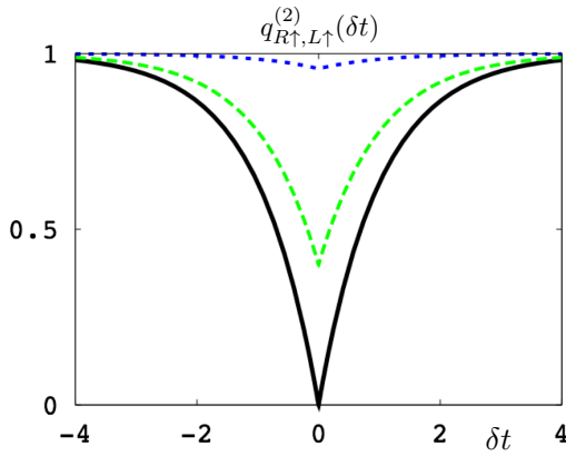
Figure 5 (Color on-line) Behavior of q_{R\uparrow,L\uparrow}^{(2)}(\delta t) as a function of \delta t (in units of \Gamma^{-1} ) for different values of spin-flipping and spin-preserving amplitudes: \gamma_{sp} = 2, \gamma_{sf} = 0 (full black curve), \gamma_{sp} = 2, \gamma_{sf} = 1.5 (dashed green curve) and \gamma_{sp} = 1, \gamma_{sf} = 0.3 (dotted blue curve). Picture taken from [18].
