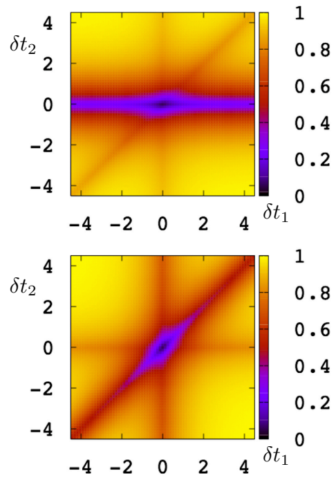
Figure 7 (Color on-line) Density plot of q^{(3)}(\delta t_1, \delta t_2) as a function of \delta t_1 and \delta t_2 (in units of \Gamma^{-1} ) for \gamma_{sp} = 1, \gamma_{sf} = 0.8 (top) and \gamma_{sp} = 2, \gamma_{sf} = 1.5 (bottom). Picture taken from [18].
