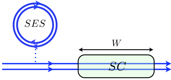
Figure 8 (Color online) Schematic view of a single electron source (SES) injecting electron and hole WPs into a IQH edge state at filling factor \nu = 2 coupled with a SC contact of length W . Picture taken from [19].
