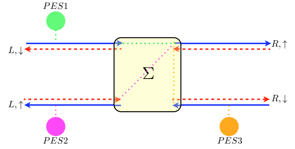
Figure 3 (Color on line) Schematic view of a QSH bar with spin up (full arrows) and spin down (dashed arrows) electrons. Dotted lines indicate the scattering processes, compatible with TRS, which affect the current in the R, \uparrow outgoing channel (see main text). Pair-electrons sources (PES) are represented with colored circles. Picture taken from [18].
