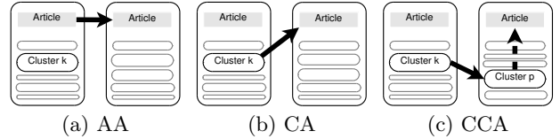
Figure 2: Different recommendation schemes.
