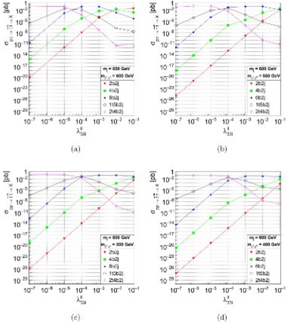
FIG. 2: Benchmark 1: production cross-section for \sigma(pp \rightarrow \tilde{l}\tilde{l} \rightarrow X) at \sqrt{s} = 14 TeV, where X = 2b2j (red triangles), 4b2j (green squares), 6b2j (blue stars), 115b2j (black empty circles) and 214b2j (pink diamonds), as a function of \lambda_{33i}^l and for m_{\tilde{l}} - m_{\chi^+} \simeq 0 GeV(a), 50 GeV(b), 100 GeV(c) and 200 GeV(d). See Tabs. II and III for the low-energy values of the MSSM parameters.
