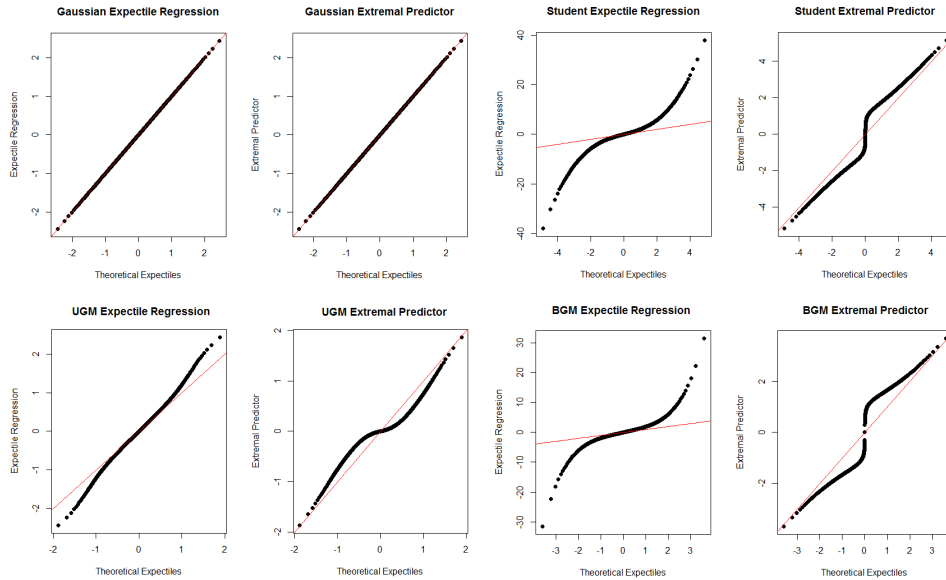
FIGURE 2. Theoretical expectiles vs expectile predictions for Gaussian, Student, UGM and BGM examples. Expectile regression appears on the left of each pair of panels, extremal predictor on the right.
