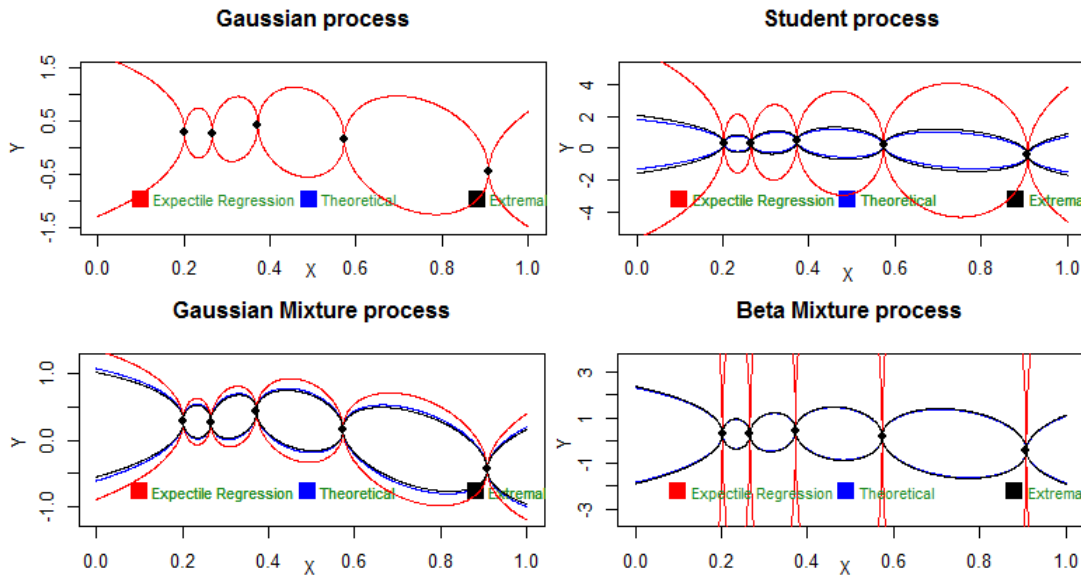
FIGURE 1. Expectile Regression Predictor in red, theoretical expectiles in blue, and Extremal Expectile Predictors in black, for a level \alpha = 0.9995
