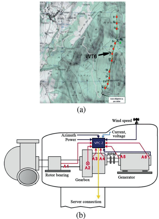
Figure 6. (a) The geographical location of the wind turbine (WT6) and (b) the accelerometers A5 and A6 installed at the front and the rear end of the generator, respectively
