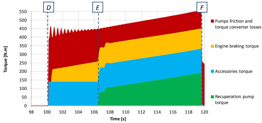
Figure 8. Solution 2: Torques distribution during a recovery phase (boom angle from 45° to 10° and container of 25t)
