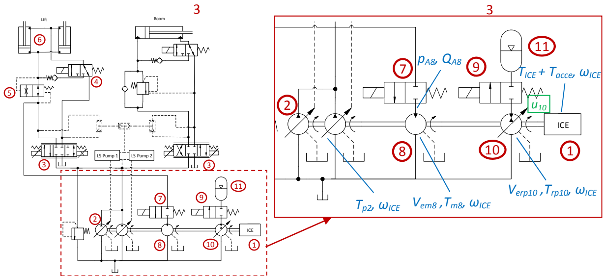
Figure 4. Hydraulic circuit with the common shaft transformer based energy recovery system
