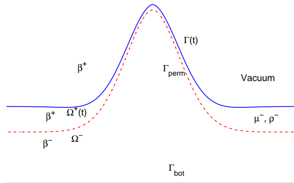
Figure 1: The solid curve (blue) is the interface \Gamma(t) and the dashed curve (red) denotes the interface \Gamma_{\text{perm}} , across which the permeability is discontinuous.
