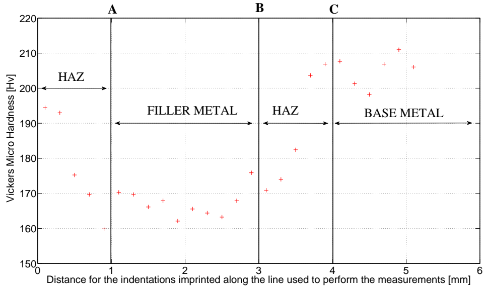
Figure 2: Microstructure and Hardness measurements performed on the welded zone of the fatigue specimen at a depth of X=0.4 mm from the outer surface.
