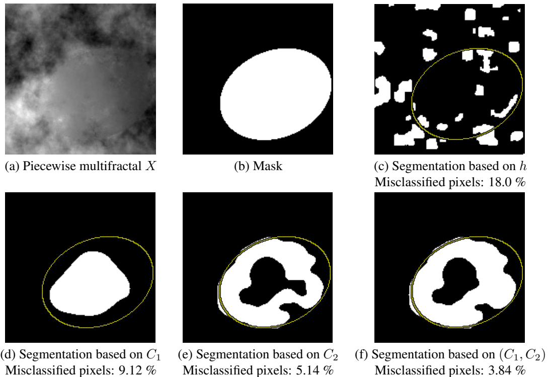
Fig. 3. Illustration of the segmentation results. The piecewise multifractal image X is presented in (a) and has been generated from the mask (b). The scalar segmentation result obtained from h is displayed in (c). The vectorial segmentation results based on C_1 , C_2 and (C_1, C_2) are respectively presented in (d), (e) and (f).
