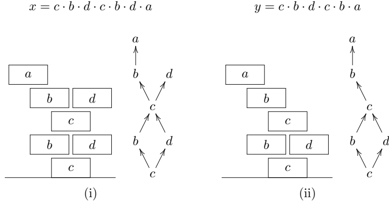
Figure 7: (i): For \mathcal{M} = \langle a, b, c, d : ac = ca, ad = da, bd = db \rangle : a trace x \notin \mathcal{V}_a (it is not pyramidal) and its associated labeled poset. (ii): a trace y \in \mathcal{V}_a and its associated labeled poset on the right.
