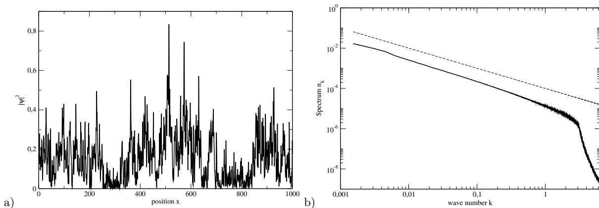
FIG. 16: a) Typical density field |\psi(x)|^2 of the solution of the MMT equation in the stationary regime for the same simulation than that of figure 15. Only a quarter of the total domain is shown for the sake of visibility. b) Spectrum n_k = \langle |\psi_k|^2 \rangle as a function of the wave number k . The statistical average is computed in the stationary regime as the mean over 4000 instantaneous spectra. The slope k^{-1} corresponding to the expected WWT turbulent spectra of direct energy cascade is shown as a dashed line for eye-guiding.
