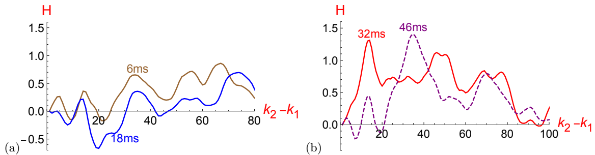
FIG. 10: k -profiles of the test function \mathcal{H} , (a) at early times t = 4 and t = 10 in units of Figs.9 , (b) at times t = 17 and t = 24 corresponding to the emergence of the first and second maximum of H(k, t) . k, t in same units as in Fig.8.
