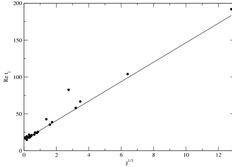
FIGURE 16. The data (black circles) for the jet formation time Re \hat{t}_j plotted as a function of J^{1/3} for all the simulations performed in this study. The data align almost perfectly along a line as suggested by the formula 4.2, that is used to fit the data (solid curve) using A_1 = 13.2 and B_1 = 14.5 .
