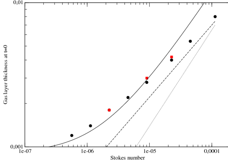
FIGURE 8. Height scale h_b/D of the gas layer as a function of the Stokes number for two values of the Reynolds number Re = 800 (red square) and Re = 2000 (black circle). The fit using equation (2.20) is shown (solid line) as well as the two scaling laws St^{2/3} (dotted line) and St^{1/2} (dashed line).
