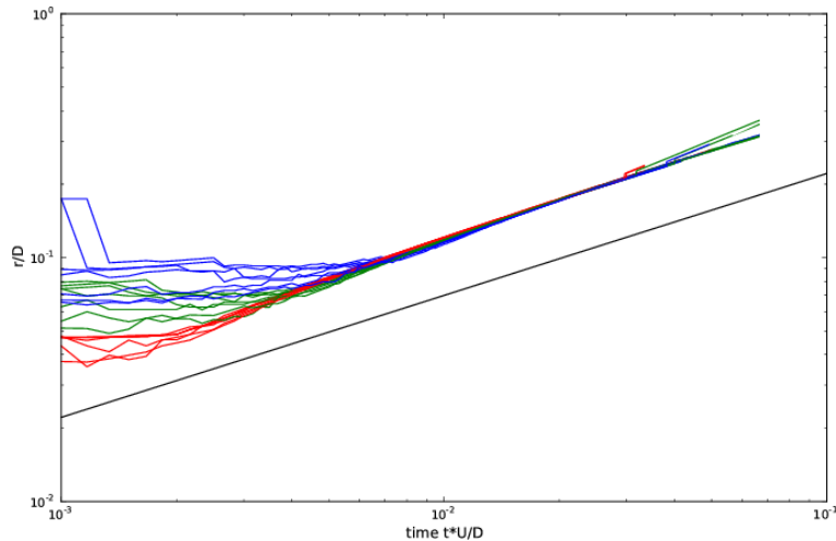
FIGURE 7. The dimensionless spreading radius defined as the radius where the velocity is maximal in the liquid, as function of the dimensionless time U_0 t/D , in a log-log plot for all the simulations performed in this study. The straight line indicates the slope 1/2 corresponding to the geometrical law r_g = \sqrt{DU_0 t} shifted below for eye guiding. As suggested by this geometrical relation, the different curves collapse all on a single one parallel to the expected law, showing that viscous, capillary and lubrication effects only alter slightly this dynamics. Differences can however be seen at short times.
