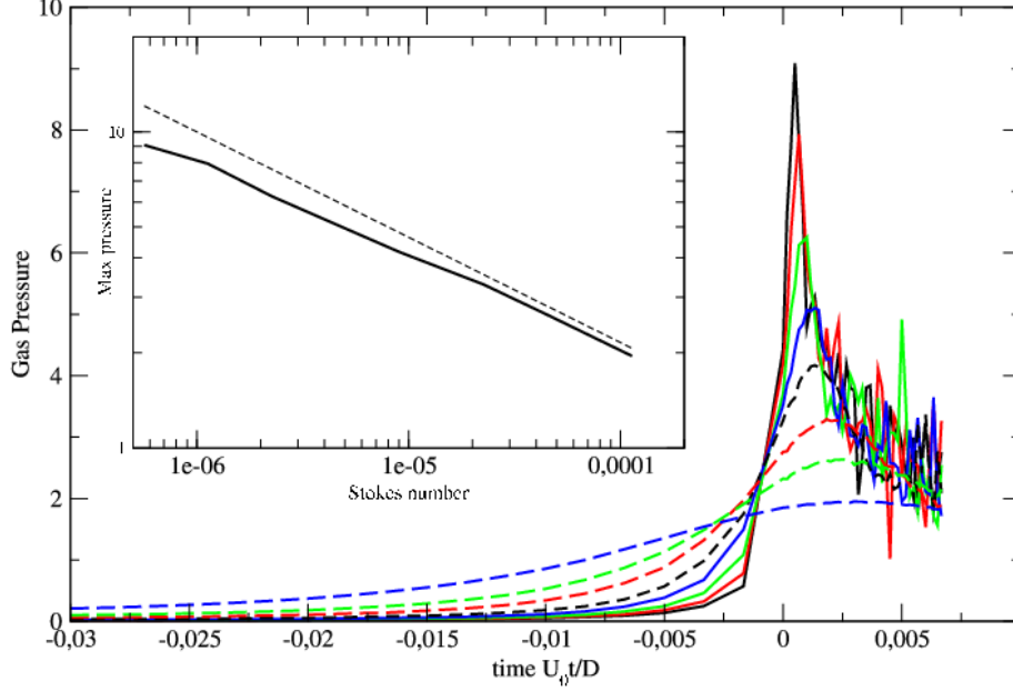
FIGURE 10. The pressure in the gas layer in the cushioning regime defined as the maximum gas pressure on the axis down the drop. The dimensionless pressure (using \rho_l U_0^2 ) is plotted as a function of the dimensionless time U_0 t/D for a fixed Re = 2000 and for varying Stokes number St = 5.66 \cdot 10^{-7} , 1.13 \cdot 10^{-6} , 2.26 \cdot 10^{-6} , 4.52 \cdot 10^{-6} , 9.05 \cdot 10^{-6} , 2.26 \cdot 10^{-5} , 4.52 \cdot 10^{-5} and 1.13 \cdot 10^{-4} , from top to bottom. The insert shows the maximum pressure over time of these curves as function of the Stokes number. The dashed line draws the expected St^{-1/3} scaling following the prediction (2.25)
