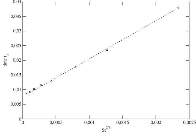
FIGURE 15. \hat{t}_j as a function of the Stokes number to the power predicted by the theory (2.23) St^{2/3} , for constant Reynolds number Re = 2000 . The dashed line indicates a linear relationship between these two quantities.
