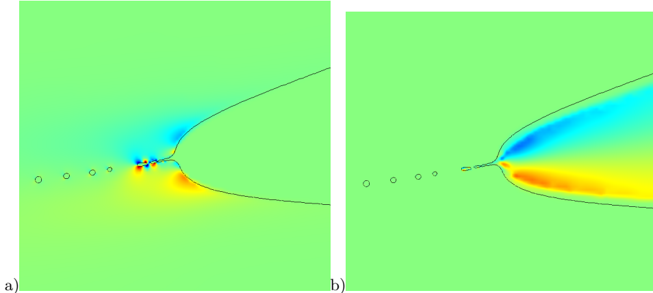
FIGURE 6. (Color online) The vorticity field corresponding to Figure 5d : a) in the liquid (the vorticity ranging here from -800 (blue) to 800 (red) in dimensionless unit) and b) in the gas (ranging from -2000 to 2000 ).
