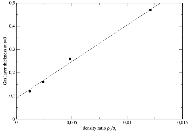
FIGURE 9. Height scale h_b/D of the gas layer as a function of \rho_g/\rho_l for St = 5.67 \cdot 10^{-7} and Re = 2000 and all other parameters as in Table 1.
