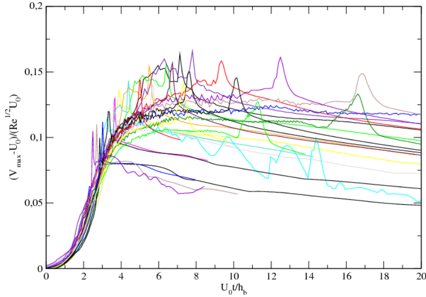
FIGURE 19. Rescaled velocities by \sqrt{Re} for all the simulations performed in this study as function of the rescaled time t/t_b , where t_b is computed using formula (2.24). The initial velocity U_0 has been subtracted at short time for clarity.
