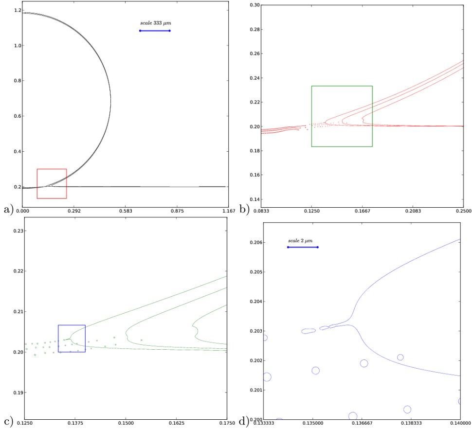
FIGURE 5. Successive zooms of the interface around the time of jet formation t_j for Re = 1000 , We = 500 , St = 2.26 \cdot 10^{-6} so that J = 0.005 . a) shows the general view; b) shows the zoom of the interface corresponding to the square traced on Figure a) and so on from b) to c) and c) to d). In the first and the last Figures, the physical scales are shown based on a D = 2 mm diameter drop for illustration. The 2 \mu m scale shown in the last Figure corresponds in fact to twenty times the smallest mesh size of the numerical simulation. Remarkably, we observe a sequence of bubble entrapment before the jet is formed, in agreement with J = (t_b/t_g)^3 \ll 1 .
