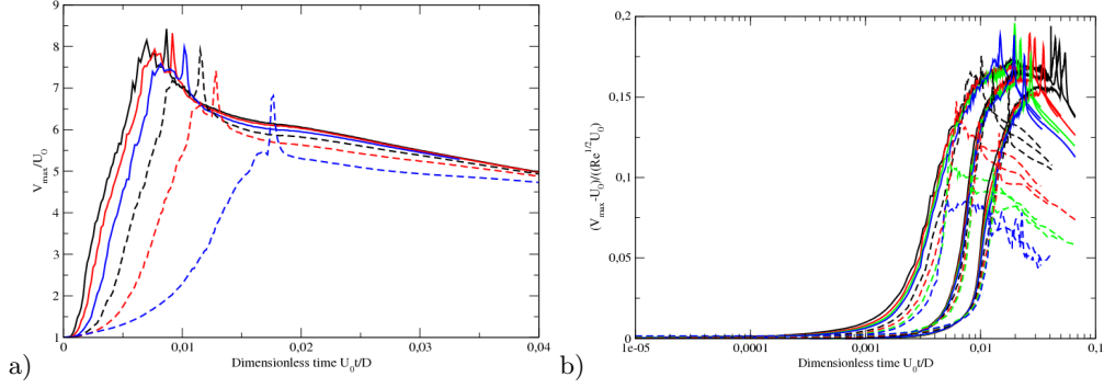
FIGURE 18. a) Maximum velocity V_{max}/U_0 as function of time for Re = 200 and for various Stokes numbers ( St = 5.65 \cdot 10^{-7} , 1.13 \cdot 10^{-6} , 2.26 \cdot 10^{-6} , 4.52 \cdot 10^{-6} , 9.05 \cdot 10^{-6} and 2.26 \cdot 10^{-5} for the curves from left to right). b) For three Stokes numbers 2.26 \cdot 10^{-6} , 9.05 \cdot 10^{-6} and 2.26 \cdot 10^{-5} the maximum velocity rescaled by \sqrt{Re} are shown for different Reynolds numbers ranging from 400 to 16000, in a log-linear plot. Three sets of curves can be identified, one for each Stokes number, from left to right as the Stokes number increases. Here, the initial velocity U_0 has been subtracted at short time for clarity.
