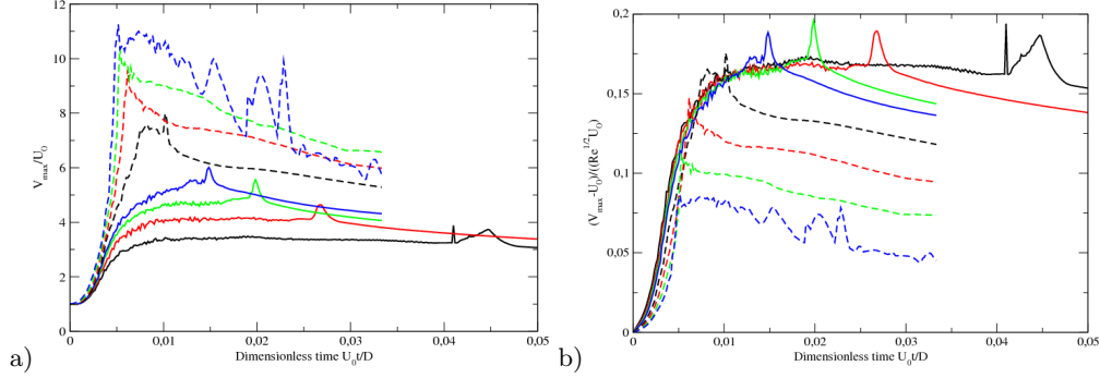
FIGURE 17. a) Maximum velocity V_{max}/U_0 as function of time for St = 2.26 \cdot 10^{-6} and for various Reynolds number ( Re = 400, 600, 800, 1000, 2000, 4000, 8000 and 16000 for the curves from bottom to top). b) Same curves where the velocity has been rescaled by the theoretical prediction \sqrt{Re} . In this case the order of the curves for increasing Reynolds numbers are reversed, ranging from top to bottom. The initial velocity U_0 has been subtracted at short time for clarity.
