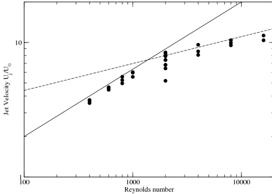
FIGURE 13. The jet velocities U_j/U_0 as function of the Reynolds number for all the simulations performed in this study, in a log-log plot. The predicted power law relation 2.4 is plotted on showing only a reasonable agreement at Reynolds number lower than 1000 (solid line). For higher Reynolds numbers another scaling appears, consistent with a Re^{1/5} law (dashed line). For Re = 2000 , where many Stokes numbers have been considered, remark a slight dependence of the velocity with the Stokes number, following the higher the Stokes number, the lower is the jet velocity.
