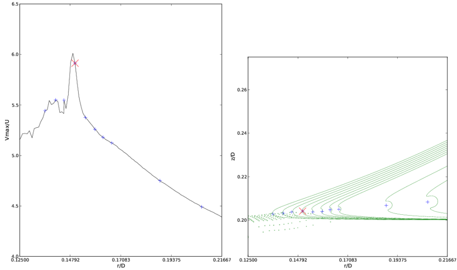
FIGURE 12. Left: the maximum velocity as a function of the radius where it is located for different times (indicated by the blue signs). Right: the interface profiles corresponding to the same time. The position at which the velocity is maximum is again marked by blue + marks. The location of the maximum velocity at time of reversal of the interface curvature, marking the beginning of jet ejection, is marked with a red \times sign.
