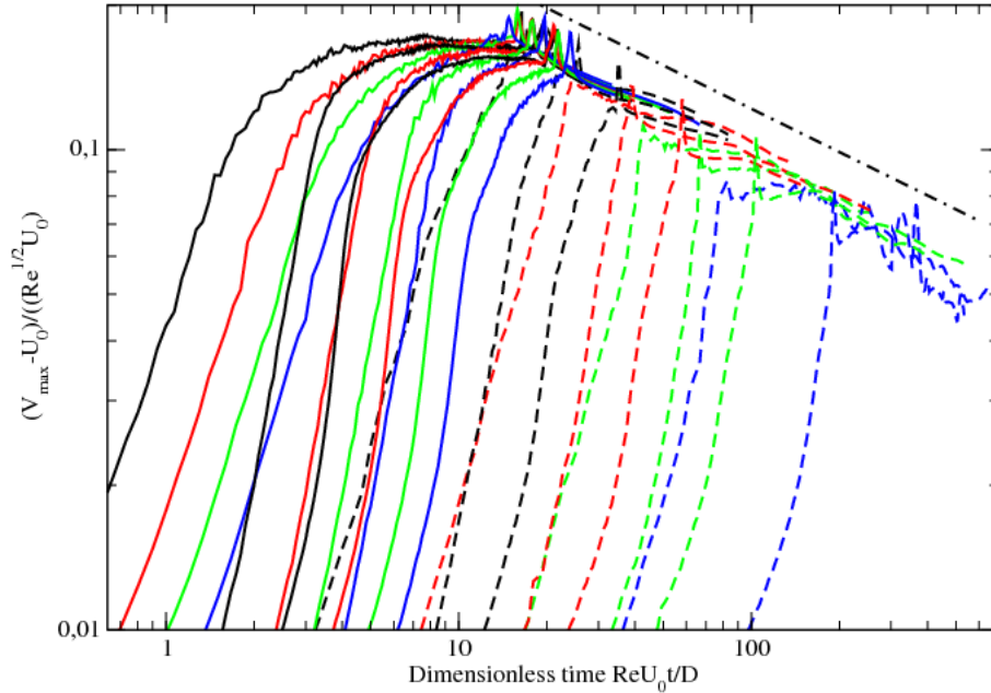
FIGURE 20. The rescaled maximum velocity V_{max}/(\sqrt{\text{Re}}U_0) shown as a function of the rescaled time \text{Re}U_0t/D based on the geometrical timescale for jet ejection t_g (see relation 2.5) in a log-log plot. The dotted-dashed line indicates the power law scaling (\text{Re}U_0t/D)^{-3/10} . The initial velocity U_0 has been subtracted at short time for clarity.
