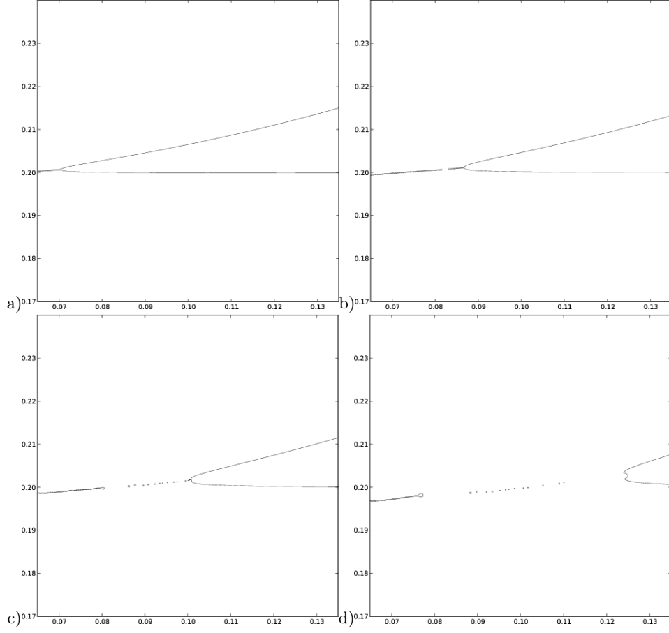
FIGURE 22. Zoom on the connexion of the upper interface of the drop with the liquid layer for \text{Re} = 2000 and \text{St} = 5.66 \cdot 10^{-7} , the other parameters being that of table 1. The interfaces are shown on time U_0 t / D = 3.67 \cdot 10^{-3} a), 5.33 \cdot 10^{-3} b), 7 \cdot 10^{-3} c) and 1.03 \cdot 10^{-2} d). The jet number J = 2.56 \cdot 10^{-3} \ll 1 and we thus observe that after the first connexion of the two interfaces on Figure a), small bubbles are created at the front of the connexion by the retraction of the thin gas layer that is still between the falling drop and the liquid film, Figure b) and c) until the jet emerges on Figure d). On the other side of the connected region, the thin air film forming the entrapped large bubble is also retracting by capillarity.
