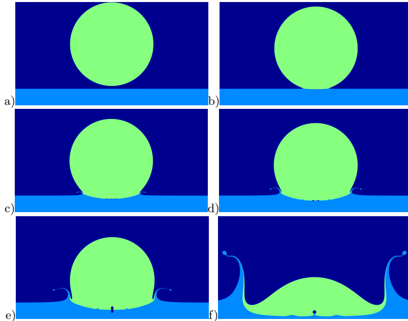
FIGURE 1. Snapshots of a droplet impacting on a thin liquid film for parameters in Tables 1 and 2, i.e. We = 500 , Re = 2000 and St = 2.26 \cdot 10^{-6} so that the jet number is J = 0.041 . For the sake of visualisation, the liquid of the droplet and of the layer have been colored in green and blue respectively, although it is the same liquid. The gas phase is colored in dark blue. The snapshots correspond to the dimensionless time U_0 t/D = -0.033, 0.0167, 0.083, 0.133, 0.217 and 0.767 respectively.
