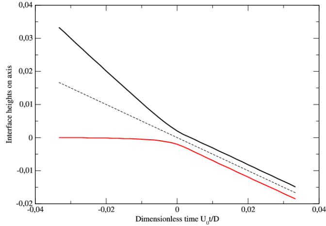
FIGURE 4. The dimensionless positions of the bottom of the droplet z_+/D and the top of the film on the axis z_-/D as a function of the dimensionless time U_0 t/D for \text{St} = 2.26 \cdot 10^{-5} , \text{Re} = 1000 and thus J = 0.5 . The dashed line represents the mean position that decreases like -0.5U_0 t .
