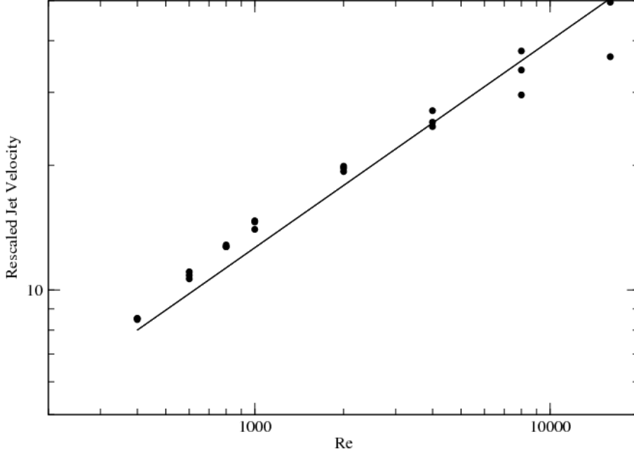
FIGURE 21. Black circles: the numerically measured jet velocity rescaled by the dependence in the J number following formula (4.6) (A_1 J^{1/3} + B_1)^{3/10} U_j / U_0 as function of the Reynolds number. The \sqrt{\text{Re}} law is drawn (solid line) showing the validity of eq. (4.6) using C1 = 0.4 .
