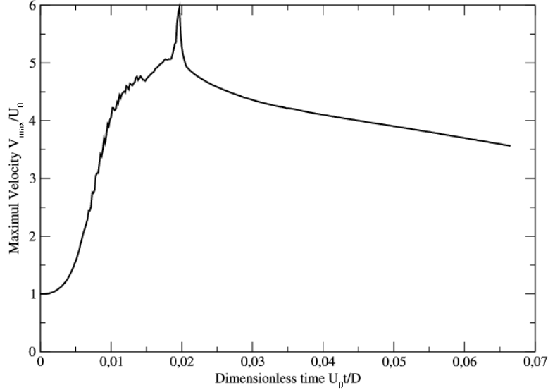
FIGURE 11. The maximum velocity V_{Max}/U_0 as a function of the dimensionless time for Re = 1000 and St = 9.05 \cdot 10^{-6} , so that J = 0.082 . Other parameters as in Table 1.
