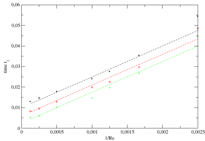
FIGURE 14. \hat{t}_j = U_0 t_j / D as a function of the inverse of the Reynolds number ( 1/Re ) for different Stokes number: black circle St = 2.26 \cdot 10^{-5} , red square St = 9.05 \cdot 10^{-6} and green diamond St = 2.26 \cdot 10^{-6} . Parallel dashed straight lines are drawn for each Stokes number for guiding the eyes.
