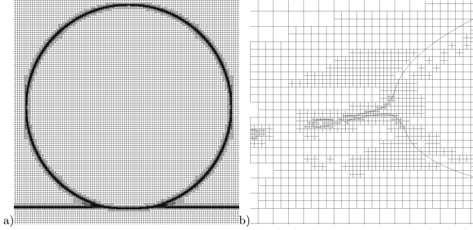
FIGURE 3. The grid refinement used in a) Figure 5a and b) Figure 5d. Here, the viscosity is twice that of Table 2, so that \text{Re} = 1000 with a gas viscosity such that \text{St} = 2.26 \cdot 10^{-6} and J = 0.005 .
