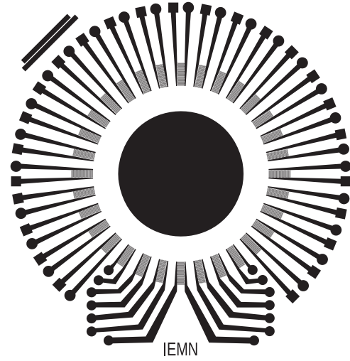
FIG. 2. Interdigitated transducer array used for generating the surface acoustic waves. The central black disk (25-mm diameter) is a gold layer acting as a mirror for interferometric measurements and materializes the maximum extent of the acoustic scene. Vector format image (available online) is used to visualize the fine structure of the electrodes.
