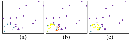
Fig. 2. Data rebalancing by ADASYN: (a) original data with two input features randomly selected from the lung tumor dataset (Section 3); (b) and (c) are two independent simulations, where more synthetic (yellow) instances have been generated for the minority class (cyan) samples which have higher difficulty in learning (on the boundary). However, due to the random nature, no points have been generated for minority class samples within the orange circle in (b).
