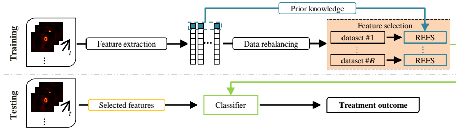
Fig. 1. Protocol of the prediction system.
