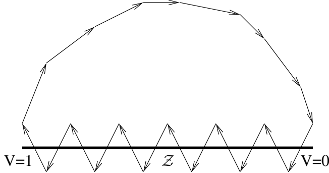
Figure 1: Strategy 2 may not provide practical stability to \mathcal{Z} when \mathcal{Z} is not reduced to a point.
