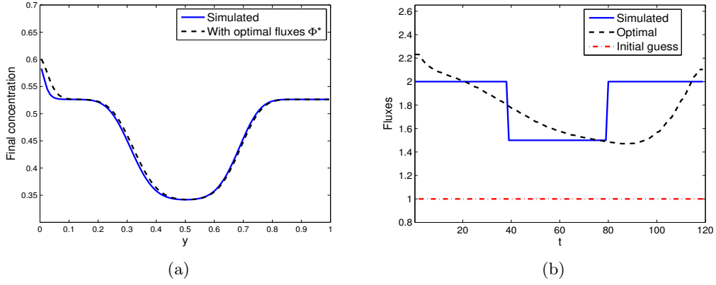
Figure 5: Reconstruction of the final concentration of the species i = 1 .
