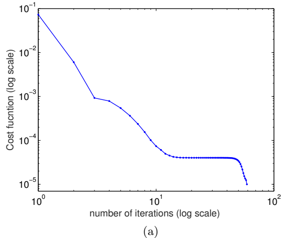
Figure 8: Convergence of the BFGS gradient descent algorithm for the minimization problem (21).
