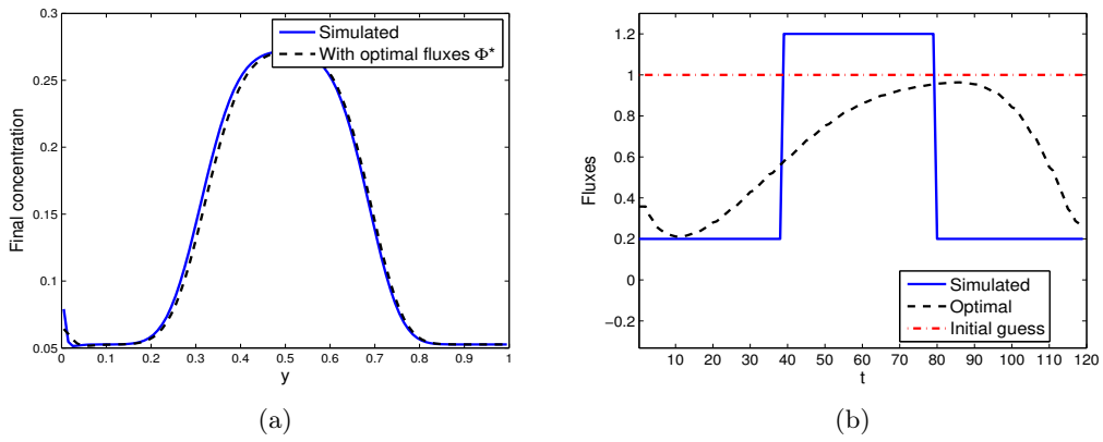
Figure 6: Reconstruction of the final concentration of the species i = 2 .
