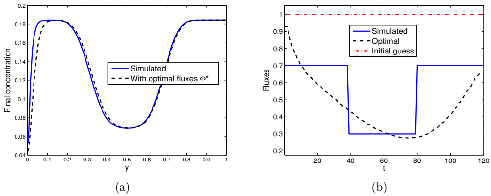
Figure 7: Reconstruction of the final concentration of the species i = 3 .
