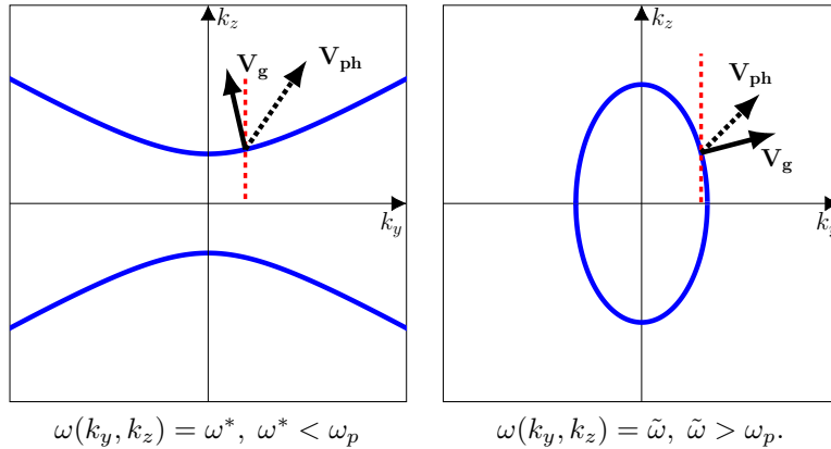
Figure 3.2: In the left figure we schematically depict level curves of the modes \pm\omega_-(0, k_y, k_z) \leq \omega_p , and in the right the level curves of the modes \pm\omega_-(0, k_y, k_z) \geq \omega_p .
