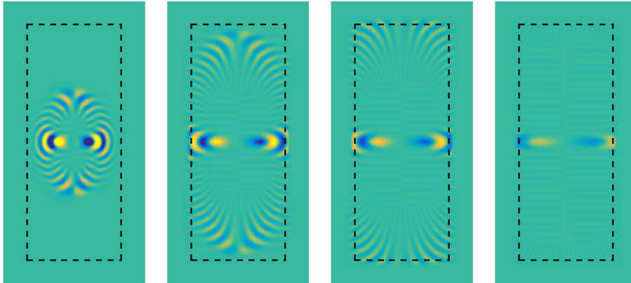
Figure 3.3: The snapshots of the field E_z computed with the help of (\text{TE})_x with the help of the new PML model (15) at t = 10, 20, 25, 40 , with the same data as in Figure 3.1.
