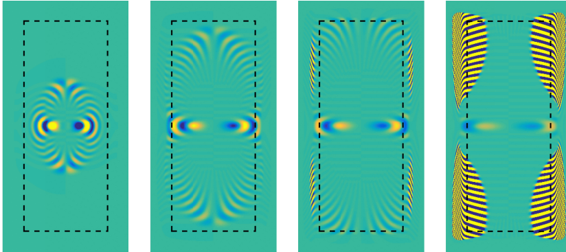
Figure 3.1: The snapshots of the field E_z computed with the help of (\text{TE})_x combined with the conventional, Bérenger's change of variables, at t = 10, 20, 25, 40 .
