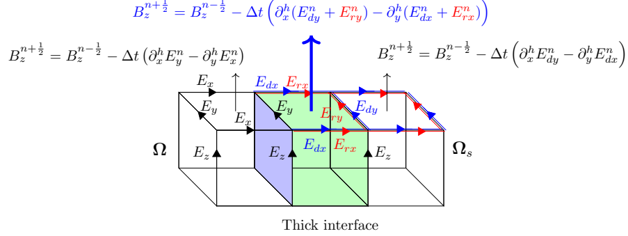
Figure 5.2: Coupling procedure for B_z . In blue we denote the boundary \Gamma_s between the regions where the split and non-split systems are solved.
