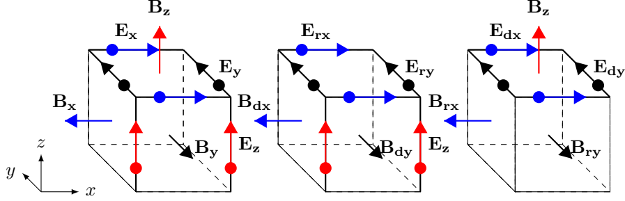
Figure 5.1: The discretization of the fields in the Maxwell and split systems.
