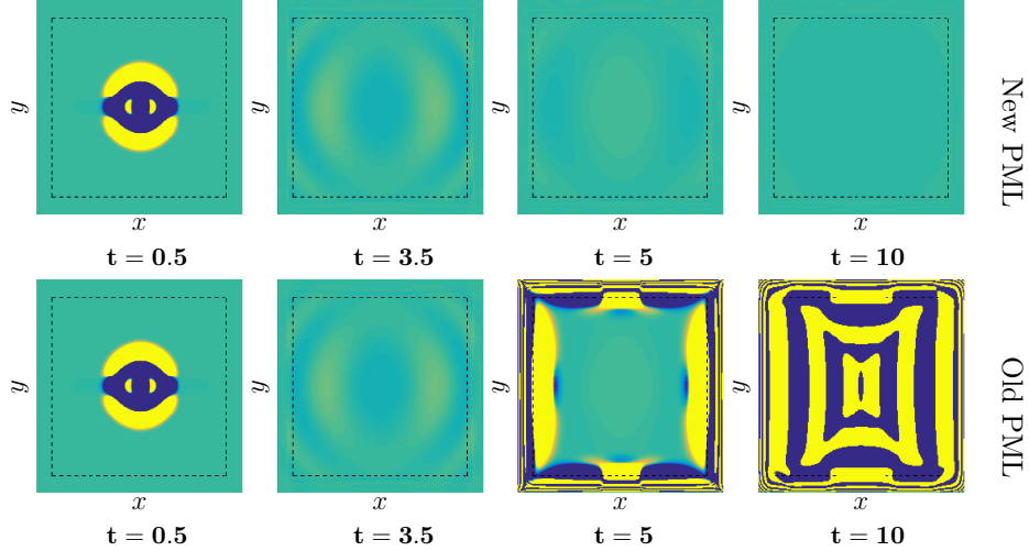
Figure 6.2: The field E_x(x, y, 0, t) computed for the experiment of Section 6.2. By a dashed line we denote a PML boundary. All figures use the same color scale.
