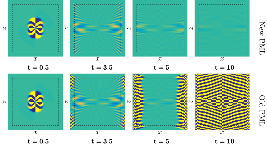
Figure 6.3: The field E_z(x, 0, z, t) computed for the experiment of Section 6.2. By a dashed line we denote a PML boundary. All figures use the same color scale.
