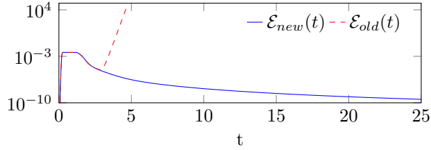
Figure 6.4: We show the approximation of a continuous energy \mathcal{E} (39) for stable and unstable (old) PMLs, computed for the experiment of Section 6.2, inside the full domain \bar{\Omega} \cup \bar{\Omega}^s \cup \Omega^{pml} .
