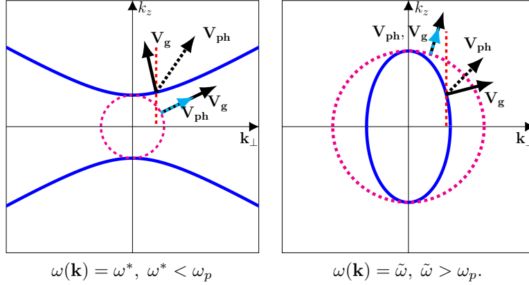
Figure 4.1: The level sets of \omega(\mathbf{k}) . The dashed circle corresponds to the mode \omega_i(\mathbf{k}) .
