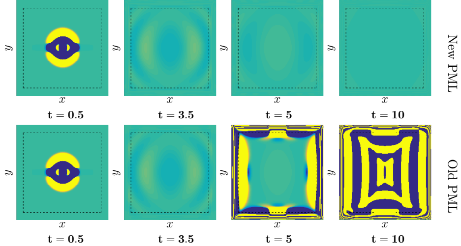
Figure 6.2: The field E_x(x, y, 0, t) computed for the experiment of Section 6.2. By a dashed line we denote a PML boundary. All figures use the same color scale.
