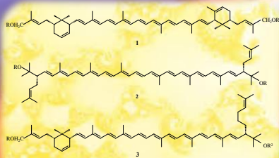
Fig. 2. Chemical structures of carotenoids produced by Arthrobacter glacialis . 1, a: R = H; b: R = Ac; Derivatized 2, a: R = H; b: R = SiMe 3 ; Derivatized 3, a: R = R 1 ; b: R = Ac; R 2 = H; c: R = Ac; R 3 = SiMe 3 .
