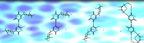
Fig. 4. Chemical structures of indochrome produced by Arthrobacter polychromogenes
