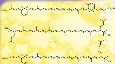
Fig. 2. Chemical structures of carotenoids produced by Arthrobacter glacialis . 1, a: R = H; b: R = Ac. Derivatized 2, a: R = H; b: R = SiMe 3 . Derivatized 3, a: R = R 1 ; b: R = Ac, R 2 = H; c: R = Ac, R 2 = SiMe 3 .
