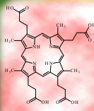
Fig. 5. Chemical structure of coproporphyrin III
