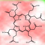
Fig. 6. Chemical structure of uroporphyrin III
