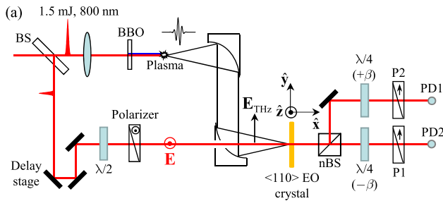
Fig. 1. (a) Experimental setup. BS, beam splitter; nBS, nonpolarizing beam splitter; P, polarizer; PD, photodiode. (b) Geometry of the experiment. (\hat{X}, \hat{Y}, \hat{Z}) , Cartesian frame of the crystal; (\hat{x}, \hat{y}, \hat{z}) , Cartesian frame of the laboratory. \mathbf{k}_{\text{THz}} (resp. \mathbf{k}_{\text{pr}} ) is the wave vector of the THz (resp. probe) pulse.
