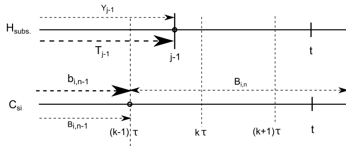
Figure B.13: The possible n th renewal cycle of component C_{si} . For H_{subst} , it may experience j - 1 th maintenance, while for soft component C_{si} , it has been renewed n - 1 times.
