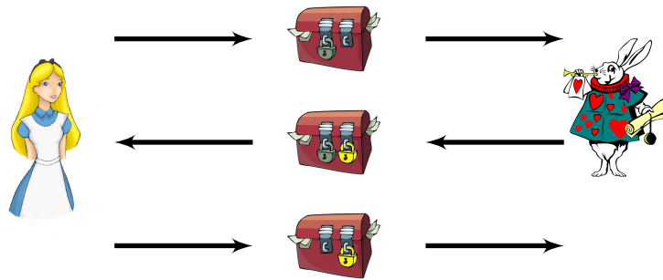
Figure 2: 3-pass Shamir protocol.
