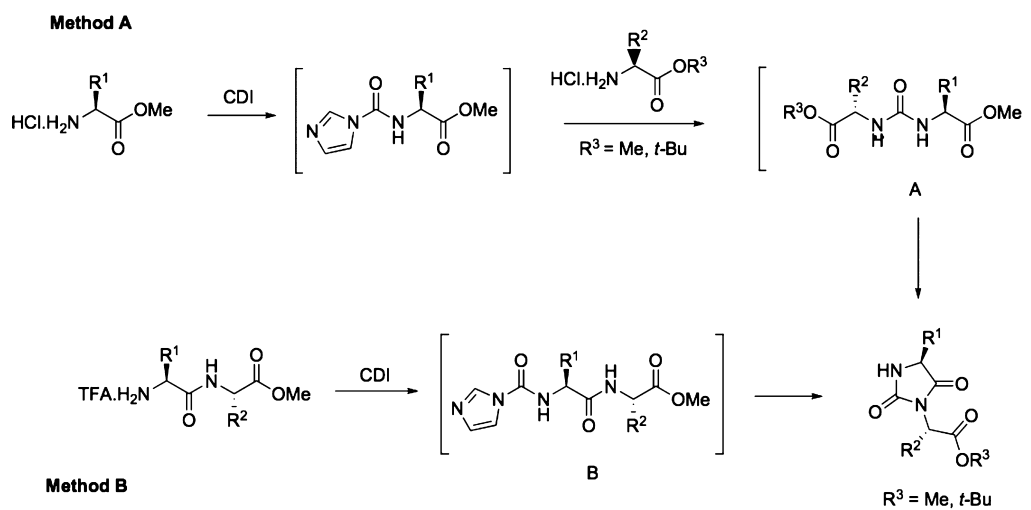
Figure 1. 5-substituted-3-(alkoxycarbonyl)alkyl-hydantoin structures.
