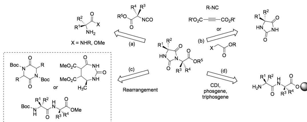
Figure 1. 5-substituted-3-(alkoxycarbonyl)alkyl-hydantoin structures.
