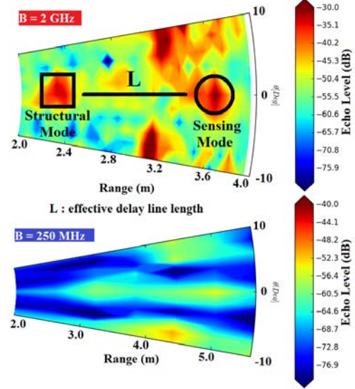
Fig. 2. 2D representation in a given elevation cut plane ( \phi=0^\circ ) of the echo level when the sensing device is replaced by an impedance of 77Ω and for 2GHz (top) and 250MHz (bottom) bandwidth modulations
