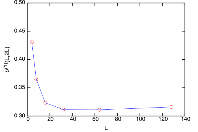
FIG. 4. The exponent b^{(1)}(L, 2L) in Eq. (38) as a function of L .
