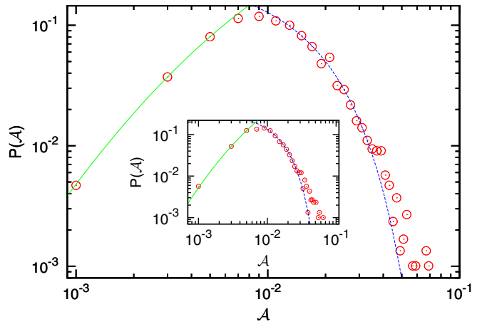
FIG. 5. Distribution P(\mathcal{A}) of the amplitudes \mathcal{A} for a BB potential, plotted with circles (numerical results). In the main figure L = 64 while the inset shows the results for L = 32 . The log-normal fit corresponding to Eq. (39) is shown for small \mathcal{A} as a solid green curve while the prediction of Eq. (47) for the right tail is shown for large values of \mathcal{A} by the dashed blue line.
