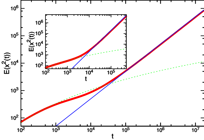
FIG. 2. Main: \mathbb{E}(x^2(t)) in a periodic Sinai model (with a periodic BB), numerical data shown as points. Also shown by the dashed line is the fit c_1 \ln^4(t) for the short-time Sinai regime along with the solid line late-time fit c_2 t . Inset: As in the main figure but for an unconstrained periodic Sinai potential.
