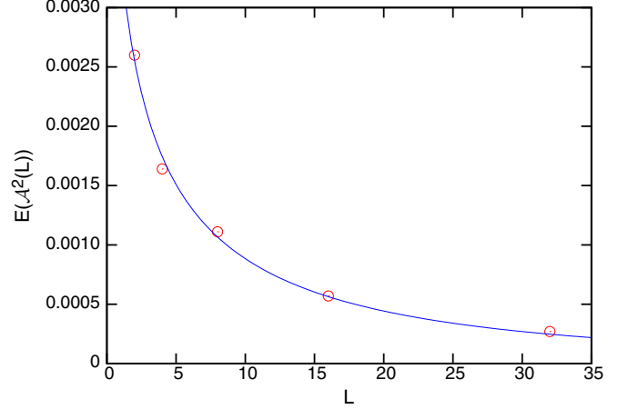
FIG. 3. The second moment of the fitted amplitudes of the power spectrum in a BB potential. Numerical results are shown as circles along with the fit of the data by a \exp(-L^b) , shown as a solid line, yielding the fitted value b = 0.37 .
