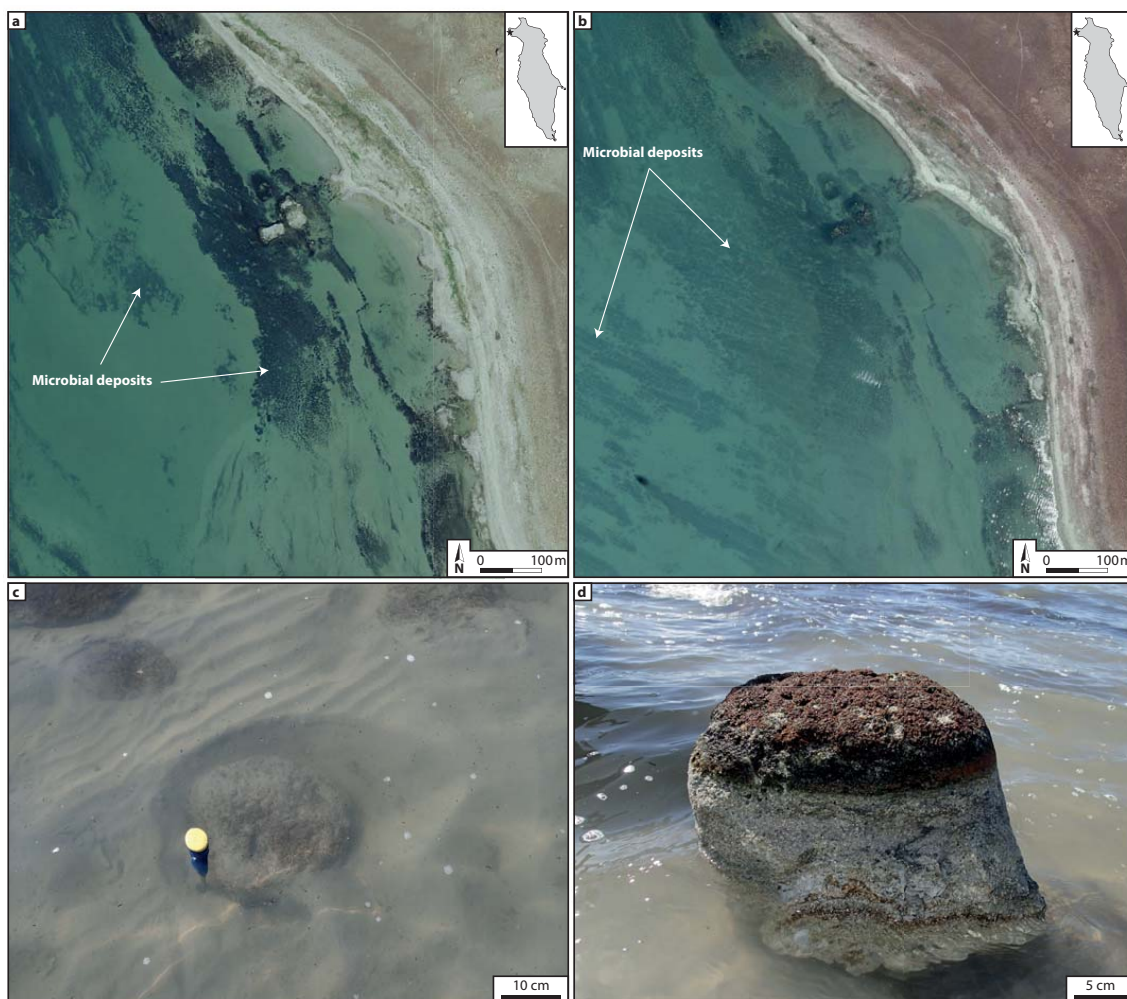
Figure 6. Illustrations of sediment removal. (a) Typical aerial/satellite images of NW Antelope Island (since 1950) with abundant microbial deposits (2014 NAIP 1 m orthophotography). (b) The same area as shown in panel a showing the burial of microbial deposits in ooid sands (Digitalglobe@images through the Garmin Birdseye software; exact date unknown but probably ca. 2013). Panels (c) and (d) depict a microbial structure that is partially buried in the ooid sand; the outcropping part (c; 3 cm high) is the only visible part; after removal from the surrounding sediment, the structure is 40 cm high (d), and the base of the column shows the attachment to an indurated substrate.
