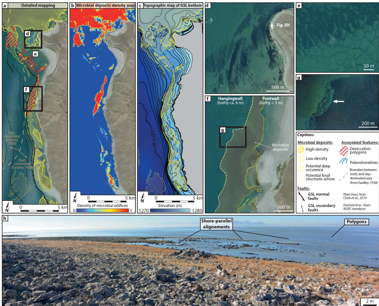
Figure 5. Detailed maps of the western side of Antelope Island. (a) Distribution and organization of the microbial deposits and sedimentary structures (2014 NAIP 1 m orthophotography). (b) Density map of the distribution of the microbial deposits. (c) Bathymetric map showing isopleths of 0.5 m. (d) Details of the microbial alignments interpreted as paleoshorelines. (e) Details of the desiccation polygons. (f) GSL major normal fault and lower limit of the microbial deposits (white dashed line); the microbial deposits are present in the footwall (yellow polygon) but not observed on the hanging wall. (g) Details of a lens-shaped detachment of the microbial deposits resulting from gliding (white arrow). (h) Photographs taken from the heights of the NW area of Antelope Island of the shore-parallel alignments of the microbial deposits on the shore.
