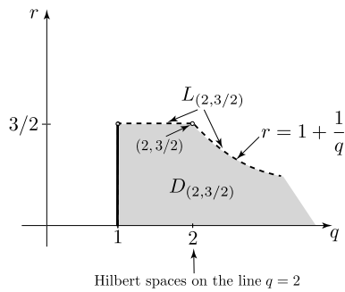
Fig. 2. The graph in (q, r) -space of the regularity of the flow of an H^{\frac{3}{2}} vector field on S^1 . The flow t \mapsto \eta(t, \cdot) of u \in C^0([0, T], H^{\frac{3}{2}}(S^1)) is in L^\infty([0, T], W^{r,q}(S^1, S^1)) , for all (q, r) \in D_{(2,3/2)} \setminus L_{(2,3/2)} . The hyperbola part of L_{(2,3/2)} has horizontal asymptote r = 1 . The flow is not in the hyperbola part of L_{(2,3/2)} .
