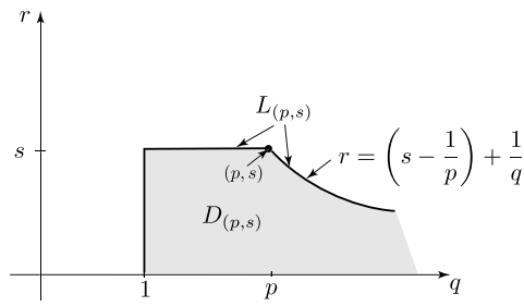
Fig. 1. The graph in (q, r) -space of the Sobolev embedding W^{s,p}(S^1) \subset W^{r,q}(S^1) . If u \in W^{s,p}(S^1) , then u \in W^{r,q}(S^1) for all (q, r) \in D_{(p,s)} including the boundary L_{(p,s)} . The hyperbola part of L_{(p,s)} has horizontal asymptote r = s - \frac{1}{p} .
