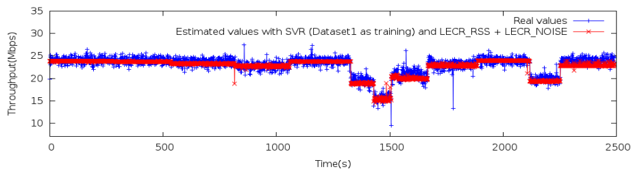
Fig. 1: Throughput estimation results obtained with the LECCR\_RSS + LECCR\_NOISE metric compared to the real throughput.
