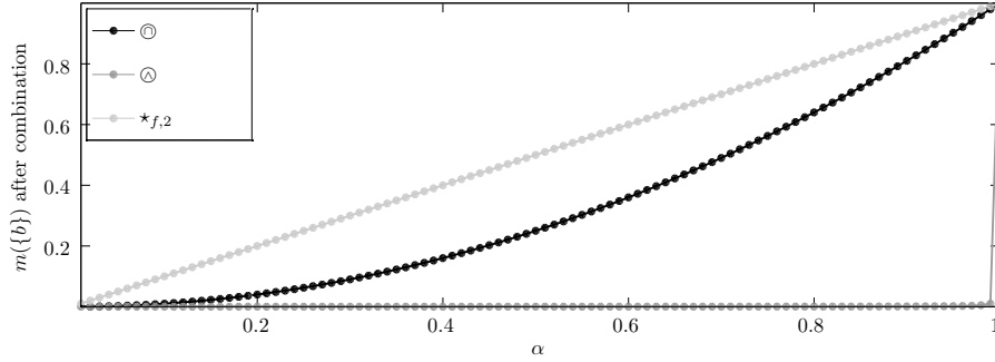
Fig. 1. Mass assigned to \{b\} after combination of m_1 = \alpha m_{\{b\}} + (1 - \alpha) m_{\{a\}} and m_2 = \alpha m_{\{b\}} + (1 - \alpha) m_{\{c\}} with \odot , \ominus and \star_{f,2} .
