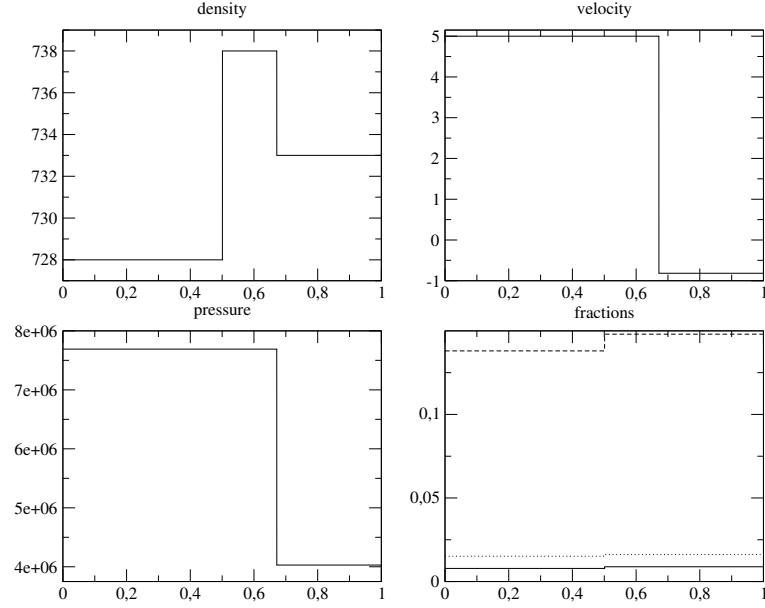
Figure 2: Analytical solution at time t = 2. 10^{-4} s for the Riemann problem of section 4.1.
