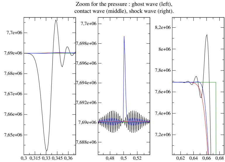
Figure 6: Comparison of the approximate solutions on a mesh with 800 cells, zoom at the wave locations for VFROENCV (red), VFROENCV-C (black), SEMI-IMP at CFL_{U+C} = 0.5 (blue). The analytical solution is in green.
