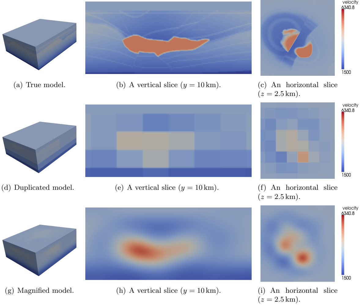
Figure 5: 3D duplicated and magnified models of the SEG/EAGE salt dome velocity model. The velocity models are built using n = 8 \times 8 \times 5 = 320 parameters, while N = 225 \times 225 \times 70 = 3543750 parameters are required for the true velocity model.
