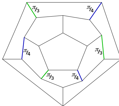
Figure 24: A geometric realisation of the dodecahedron \mathcal{D}_3 with a rotational symmetry of order 3. All unlabelled edges have dihedral angles \pi/2 , the labelled ones have dihedral angles \pi/3 and \pi/4 in the alternating fashion.
