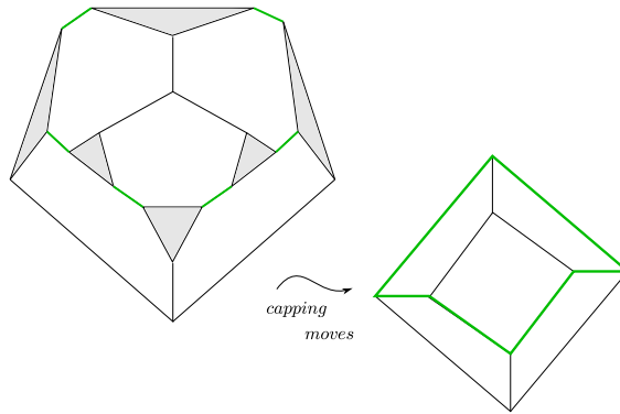
Figure 22: The sequence of I - H and capping moves for a dodecahedron
