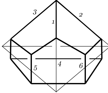
Figure 10: A tetrahedron of type t|a1234|p56
