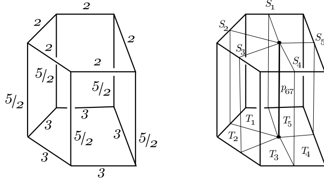
Figure 14: A geometric realisation of the prism \Pi with given dihedral angles, and its decomposition into generalised tetrahedra
