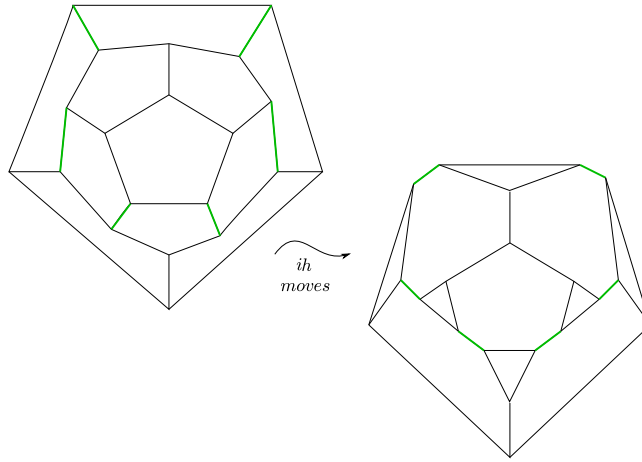
Figure 21: The sequence of I - H and capping moves for a dodecahedron
