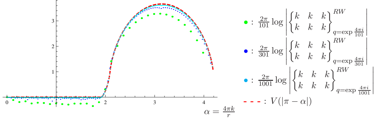
Figure 25: Values of the quantum 6j-symbol and V(\alpha) .
