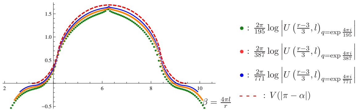
Figure 26: Values of U(\frac{r-3}{3}, l) and V(\beta) .
