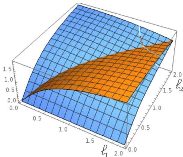
Figure 16: The dihedral angles of the tetrahedron T_4 as functions of edge lengths \ell_1 and \ell_2 (the graph is symmetric under exchanging \ell_1 and \ell_2 )
