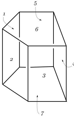
Figure 3: A pentagonal prism II
