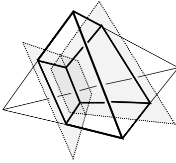
Figure 7: A prism-truncated tetrahedron
