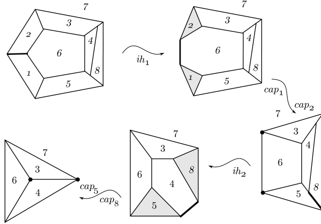
Figure 18: Another sequence of I - H and capping moves reducing the pleated prism \mathcal{P} to a tetrahedron
