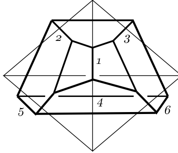
Figure 12: A tetrahedron of type t|a14|p2356
