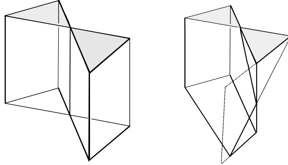
Figure 17: Some examples of “butterfly” generalised tetrahedra
