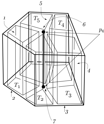
Figure 13: A geometric decomposition of \Pi into tetrahedra T_i , i = 1, \dots, 5 , of type t|a12345|p6
