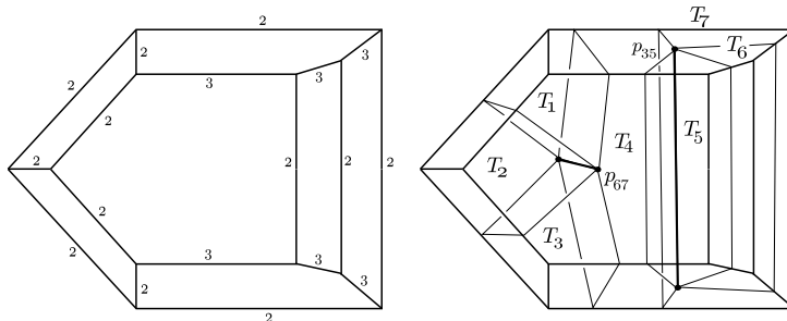
Figure 15: A geometric realisation of the prism \mathcal{P} with given dihedral angles, and its decomposition into generalised tetrahedra
