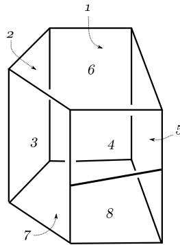
Figure 5: A pentagonal pleated prism \mathcal{P}
