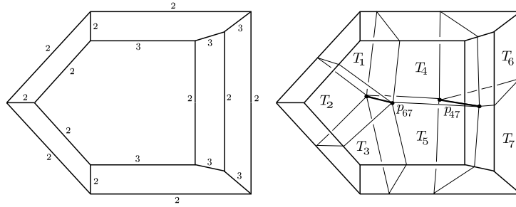
Figure 19: A geometric realisation of the pleated prism \mathcal{P} with given dihedral angles, and its decomposition into generalised tetrahedra
