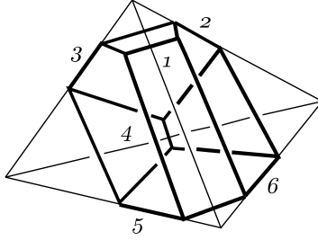
Figure 9: A tetrahedron of type t|a2356|p14
