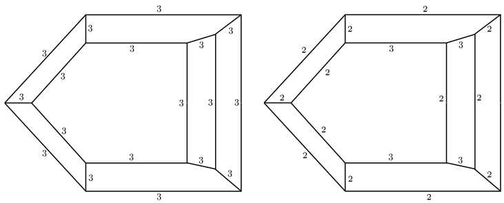
Figure 20: Various pleated prisms with volumes \sim 9.52855 (left: this one has all ideal vertices) and \sim 1.792925 (right: it has many right angles and thus considerably smaller volume)
