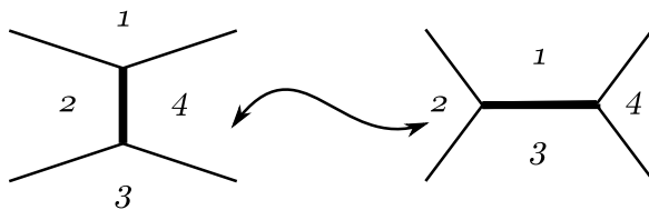
Figure 1: An I - H move
