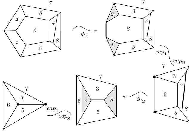
Figure 6: A sequence of I - H and capping moves applied to the pleated prism \mathcal{P}
