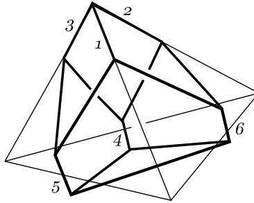
Figure 11: A tetrahedron of type t|a123|p456
