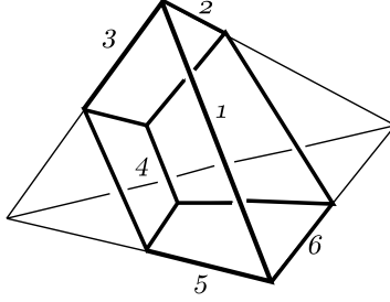
Figure 8: A tetrahedron of type t|a12356|p4
