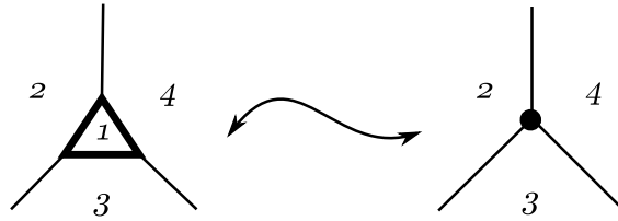
Figure 2: A “capping” move
