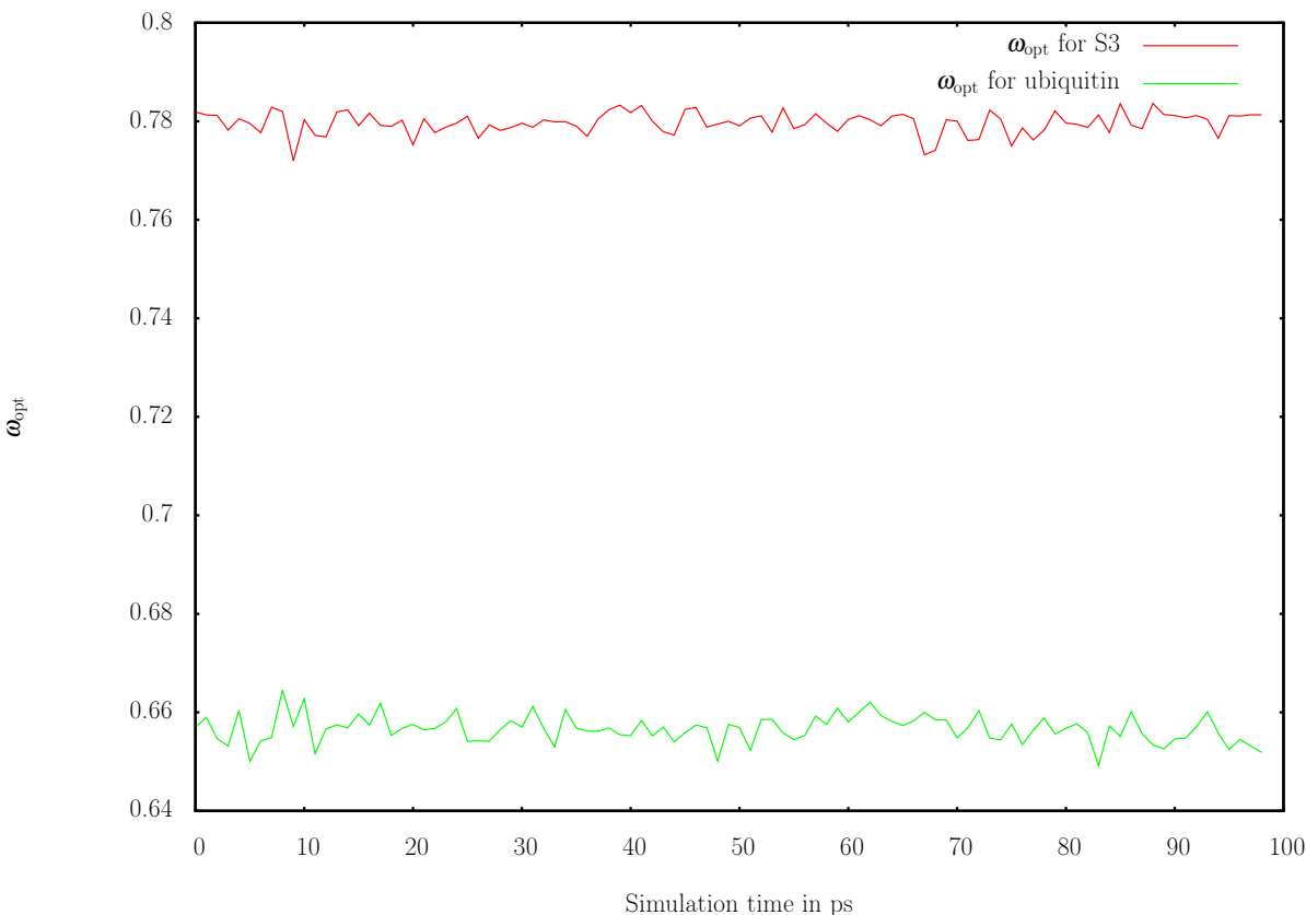
Figure 4: Evolution of \omega_{\text{opt}} for S3 and ubiquitin.
