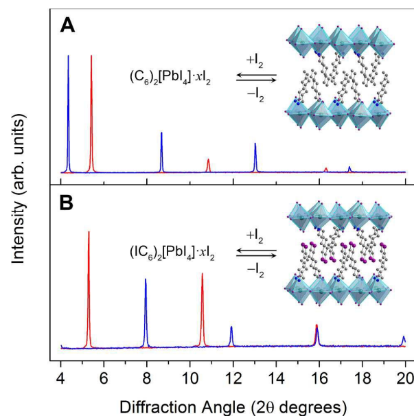
Figure 1. (A) Powder X-ray diffraction (PXRD) patterns of (C_6)_2[PbI_4] (red) and (C_6)_2[PbI_4] \cdot xI_2 (blue). Inset: X-ray crystal structure of (C_6)_2[PbI_4] . (B) PXRD patterns of (IC_6)_2[PbI_4] (red) and (IC_6)_2[PbI_4] \cdot xI_2 (blue). Inset: X-ray crystal structure of (IC_6)_2[PbI_4] . Green, purple, blue, and grey spheres represent Pb, I, N, and C atoms, respectively. Disordered atoms and hydrogen atoms are omitted for clarity.
