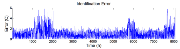
Figure 4: Identification errors
