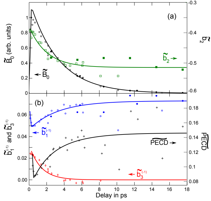
Figure 3: Temporal evolution of \tilde{b}_{odd}^{(-1)} , \tilde{b}_2 and \tilde{b}_0 with empty markers data recorded on (1R)-(-) enantiomer and filled ones on (1S)-(+ enantiomer (with a sign inversion on the \tilde{b}_{odd}^{(+1)} ). (a) \tilde{b}_0 in black, \tilde{b}_2 in green, (b) \tilde{b}_1^{(-1)} in blue, \tilde{b}_3^{(-1)} in red and \overline{\text{PECD}} in black. Table 1 summarizes the time constants extracted from the fits (see SI). When the population in 3s state starts to be less than 10% (delay \geq 7 ps), the normalisation by a small \tilde{B}_0 increases the dispersion of the normalised coefficients.
