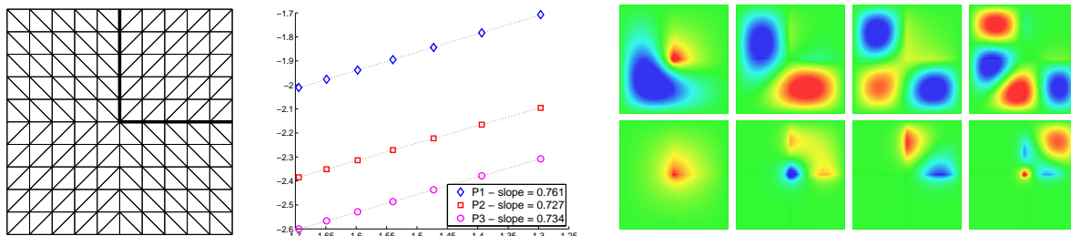
FIGURE 1 – Left : coarse symmetric mesh. Centre : relative error vs. h (log-log scale) for \lambda_1 \approx 13.2391 . Right : eigenfunctions associated with \lambda_1^h, \dots, \lambda_4^h (top) and \lambda_{-1}^h, \dots, \lambda_{-4}^h (bottom).
