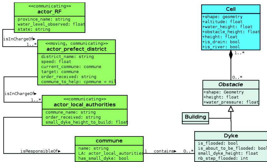
Figure 5. UML class diagram of the model
