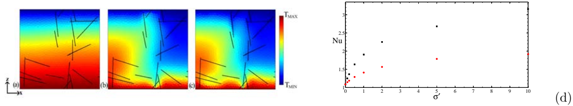
Figure 1: Temperature fields at steady state for \sigma' = 0.1 (a), 5 (b) and 10 (c), and Nu as a function of \sigma' (d) for \text{Ra}_m = 41.5 . Data are for \rho' = 4 in (a-c) and for \rho' = 1 (red symbols) and 4 (black symbols), in (d).
