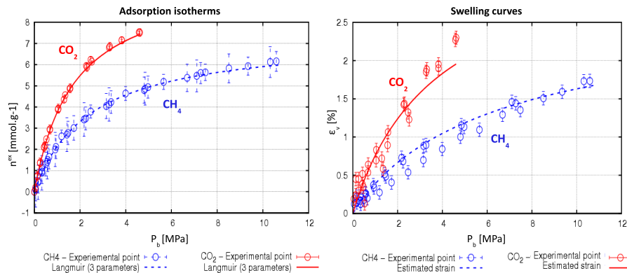
Figure 1: Adsorption isotherms and swelling curves. Thanks to the adsorption isotherms measured experimentally ( CH_4 and CO_2 ), the deformations predicted by the model extended correspond to the deformations measured by the experimental set-up.
