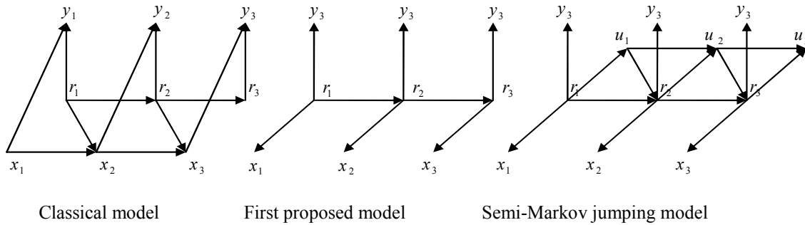
Figure 1. Dependence graphs of the classical Markov switching linear system, the proposed Markov switching system, and the proposed semi- Markov switching system.
