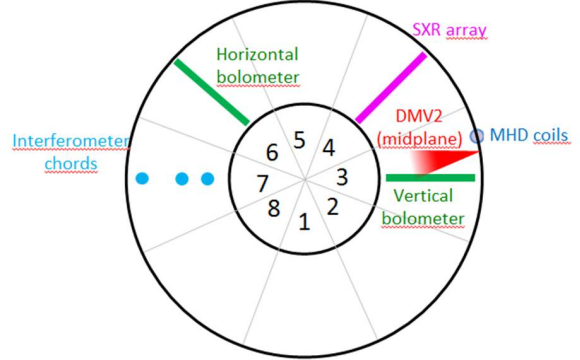
Figure 3. Schematic machine view from the top showing the DMV2 and interferometer chords
