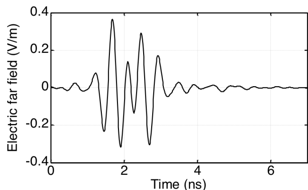
Fig. 2. Measured electric far field backscattered by the patch antenna in the boresight direction in the time domain for a Gaussian excitation signal.
