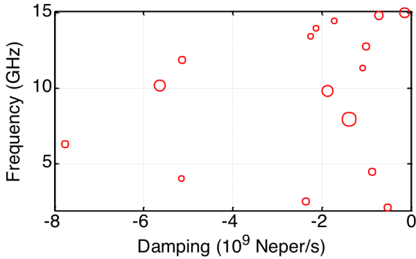
Fig. 20. Poles extracted from the windowed electric far field backscattered by the UWB antenna using a |R|/|\sigma| weighting.
