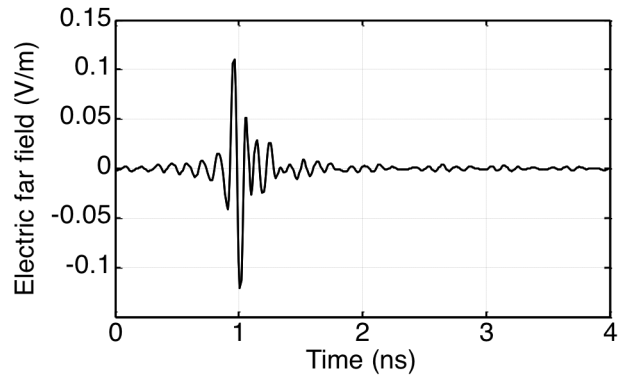
Fig. 19. Measured electric far field backscattered by the UWB antenna in the boresight direction ( \theta = \varphi = 90^\circ ) in the time domain for a Gaussian excitation signal.
