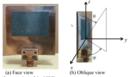
Fig. 18. Presentation of the UWB antenna.
