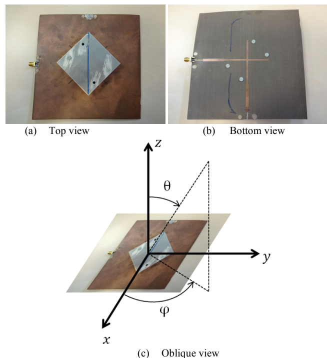
Fig. 1. Presentation of the patch antenna.
