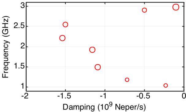
Fig. 6. Poles extracted from the windowed electric far field backscattered by the patch antenna, represented in the complex plane using a |R|/|\sigma| weighting.
