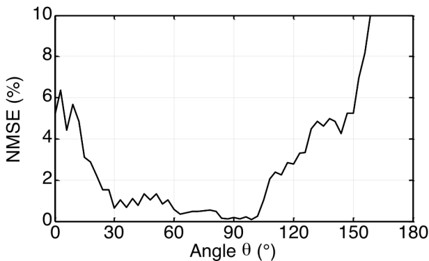
Fig. 21. The Normalized Mean Square Error of the reconstructed response of the UWB antenna using the same set of poles as a function of the angle of incidence \theta .
