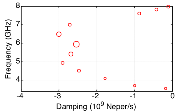
Fig. 15. Poles extracted from the windowed electric far field backscattered by the helical antenna, represented in the complex plane using a |R|/|\sigma| weighting.
