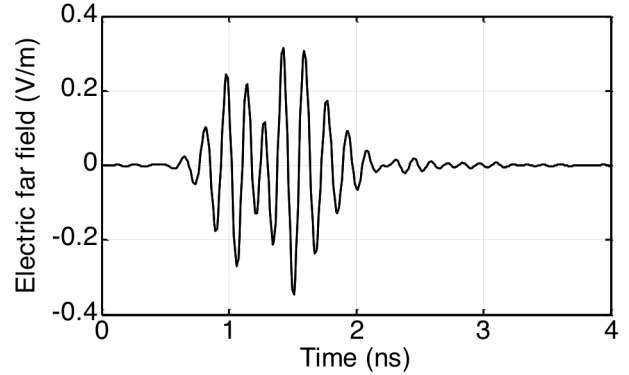
Fig. 14. Measured electric far field backscattered by the helical antenna in the boresight direction in the time domain for a Gaussian excitation signal.
