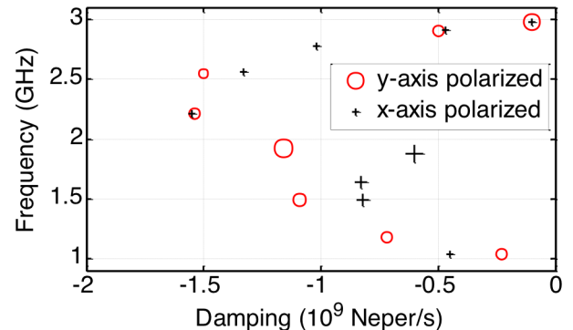
Fig. 11. Poles extracted using x-axis and y-axis polarized incident wave in the boresight direction, represented in the complex plane.
