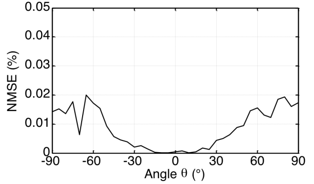
Fig. 7. The Normalized Mean Square Error of the reconstructed response using the same set of poles as a function of the angle of incidence.
