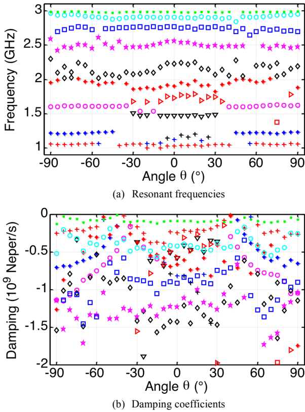
Fig. 12. Poles extracted from the measured electric far field backscattered by the patch antenna as a function of \theta , \varphi = 0^\circ , x-axis polarized incident wave.
