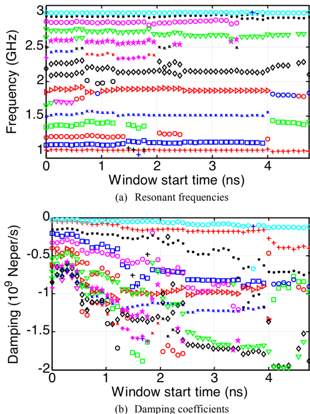
Fig. 3. The MPM applied on a decreasing window with a fixed end time equal to 6 ns.
