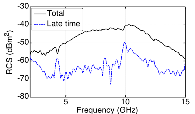
Fig. 23. Measured Radar Cross Section of the UWB antenna (solid) and measured Radar Cross Section of the UWB antenna linked to the late time response only (dashed).
