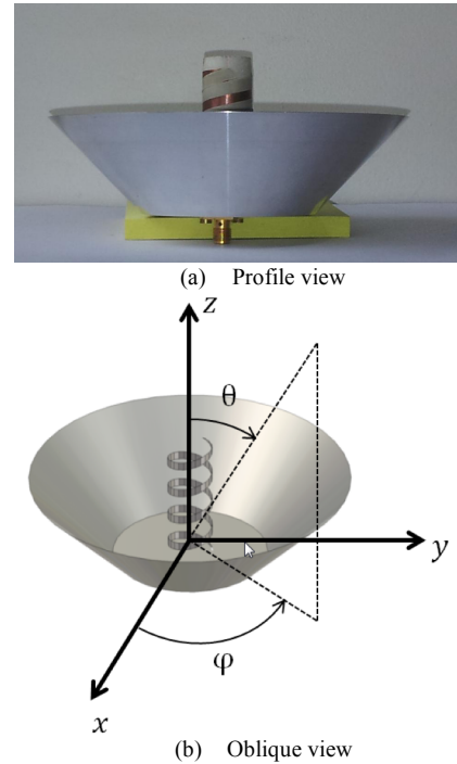
Fig. 13. Presentation of the helical antenna.
