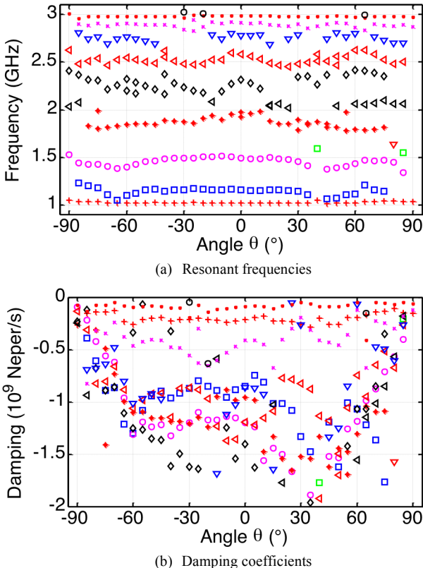
Fig. 9. Poles extracted from the measured electric far field backscattered by the patch antenna as a function of \theta ( \varphi = 90^\circ plane).
