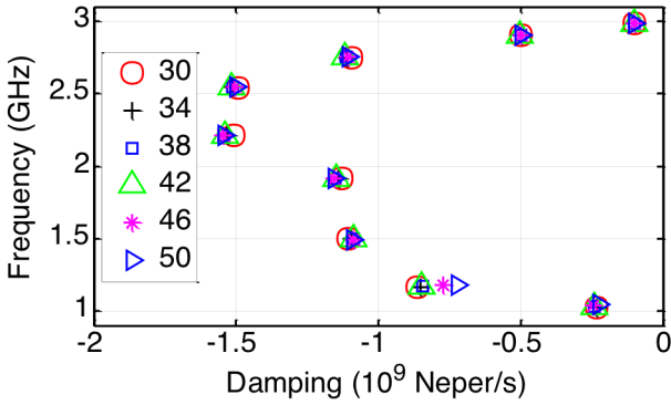
Fig. 5. Poles extracted from the windowed electric far field backscattered by the patch antenna for several N values from 30 to 50, represented in the complex plane.
