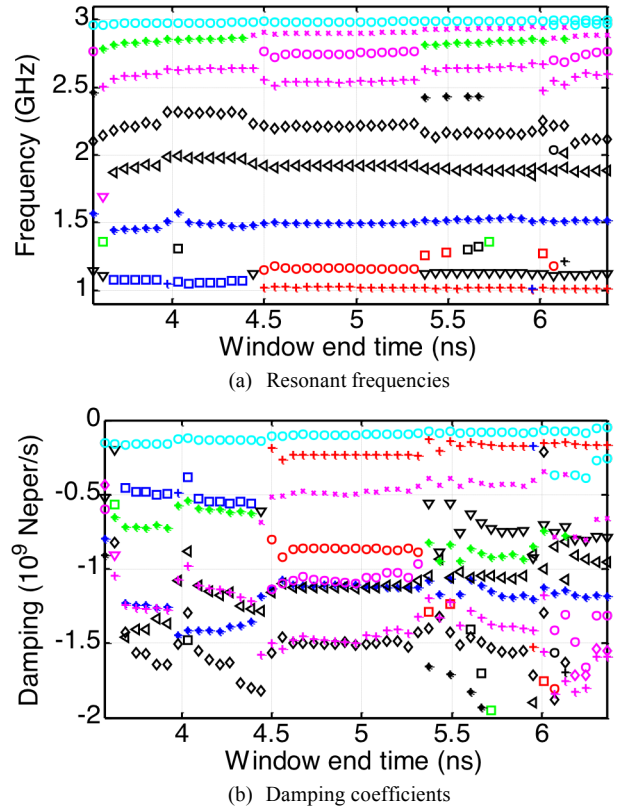
Fig. 4. The MPM applied on an increasing window with a fixed start time equal to 2.4 ns.
