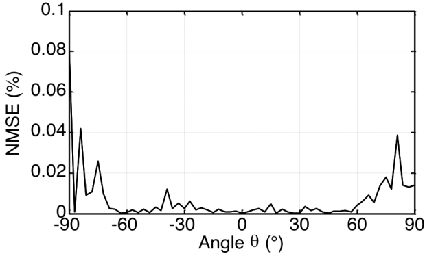
Fig. 16. The Normalized Mean Square Error of the reconstructed response of the helical antenna using the same set of poles as a function of the angle of incidence \theta .
