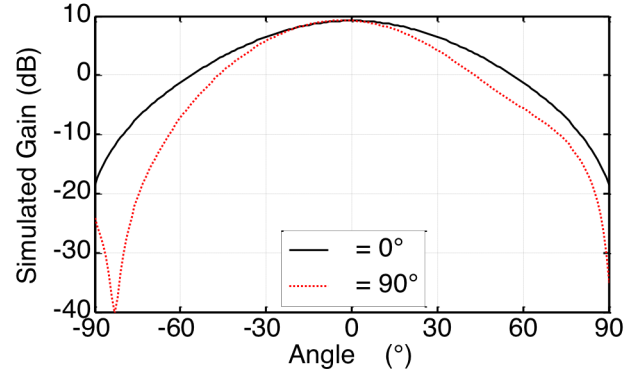
Fig. 10. Simulated radiation pattern of the patch antenna for two planes: \varphi = 0^\circ and \varphi = 90^\circ at 2 GHz.
