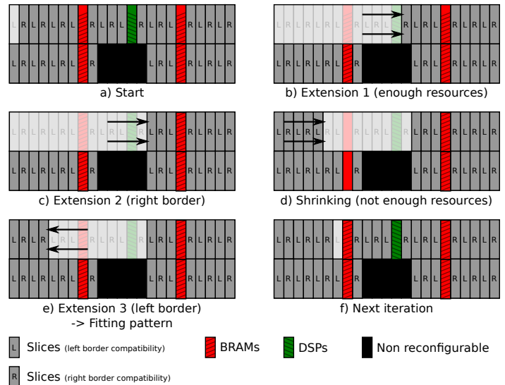
Fig. 2. Example of iterative identification of fitting patterns: needs 8 slice columns, 1 BRAM column and 1 DSP column
