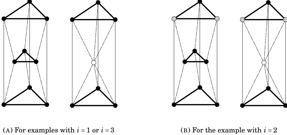
FIGURE 5. The spherical vertices are in black, the parabolic vertices are in white, and the loxodromic vertices are in gray.
