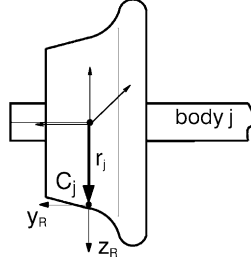
Fig. 6. Definition of wheel profile and wheel radius.
