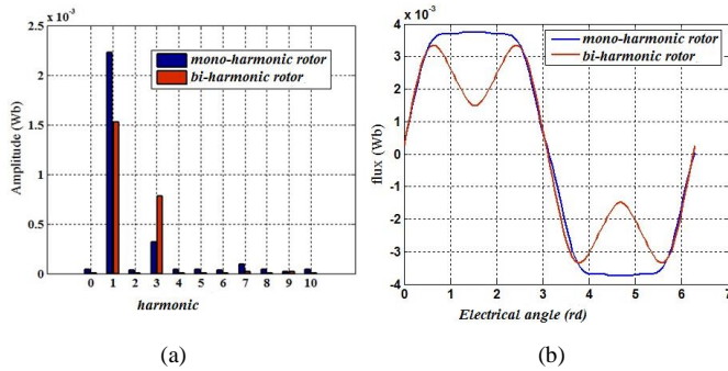
Fig.2. Comparison of flux between mono-harmonic and bi-harmonic rotors. a) Spectrum of flux. b) flux waveform.
