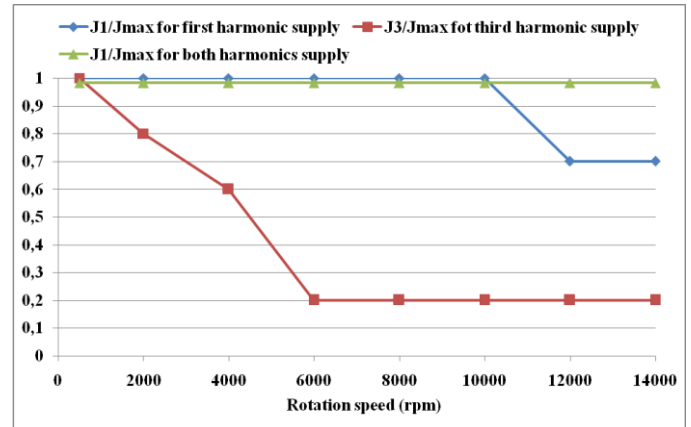
Fig. 9. Current supply for each control strategy ( J_{max}=10 A/mm^2 )
